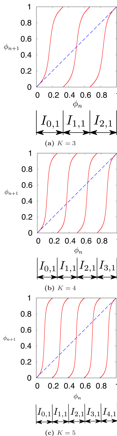
FIG. 3. The solid lines correspond to the transformation \tilde{S}_{K,1} , which has exact topological conjugacy with the SGB transformation S_{K,1} , where K = 3, 4 , and 5. The dashed line corresponds to the line \phi_{n+1} = \phi_n . (a), (b), and (c) correspond to the case of K = 3, 4 , and 5, respectively.
