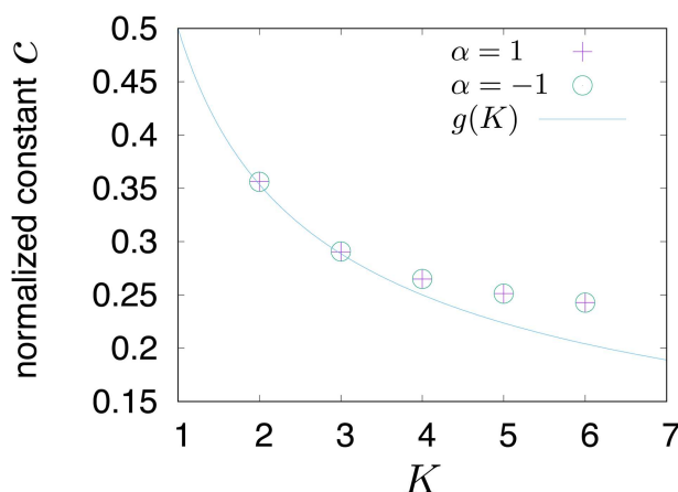
FIG. 6. Relation between normalization constant c(K) and parameter K . The function g(K) is rewritten as g(K) = \frac{1}{2\sqrt{K}} .
