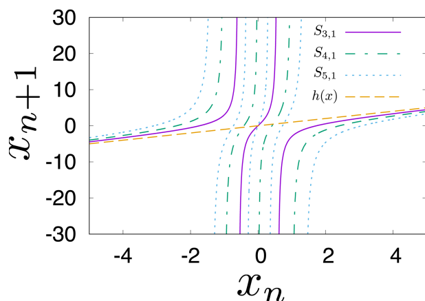
FIG. 1. Return maps of S_{3,1} , S_{4,1} , and S_{5,1} . The function h(x) = x represents the set of fixed points.
