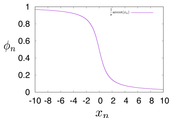
FIG. 2. Relation between x_n and \phi_n .
