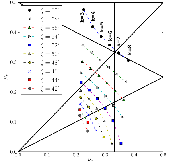
Figure 2: Cell tunes plot by lattice parameter searching with cell number N = 10 , k range 3.0-8.0, \zeta up to 60°. Normal structure resonances up to 3rd order are plotted
