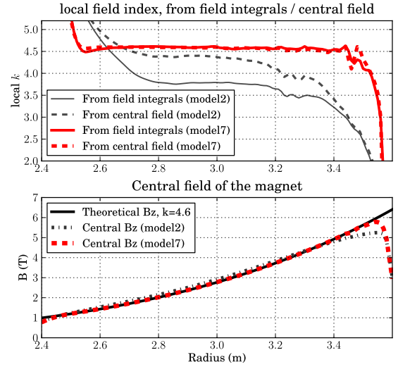
Figure 8: (top) local field index calculated from field integrals and central field of the magnet sector; (bottom) central field distribution along the radius, comparison to theoretical value from scaling law
