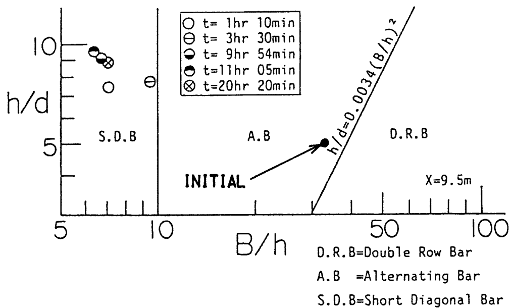
Fig. 7. Regime of meso-scale bed configuration.
