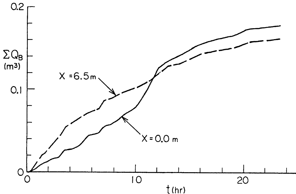
Fig. 9. Temporal variation in the accumulated sediment discharge.
