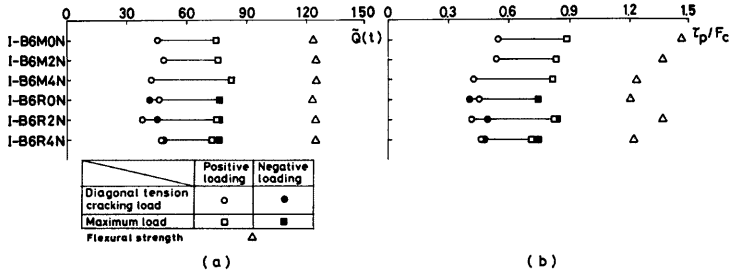
Fig. 12. Shear capacity of beam-to-column connection.
