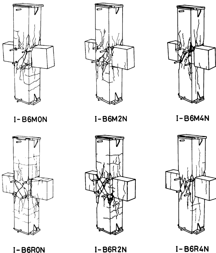
Fig. 3. Crack observation.
