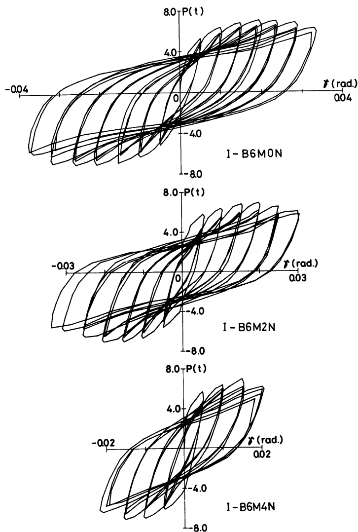
Fig. 5. Hysteresis loops.
