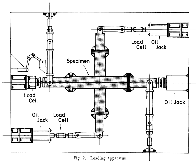
Fig. 2. Loading apparatus.
