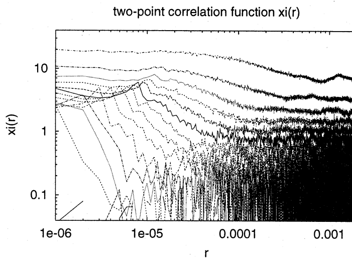
Figure 2: Evolution of correlation function \xi(r) at t = \frac{5}{64}\ell , \ell = 3, 4, \dots, 17 (from bottom to top). System size N = 2^{14} , Initial condition: x_i = \text{random} , v_i = 0 .
