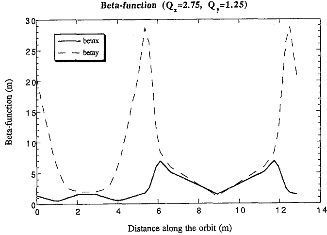
Fig. 4. \beta -functions in the half circumference for the operating point of (2.75, 1.25).
