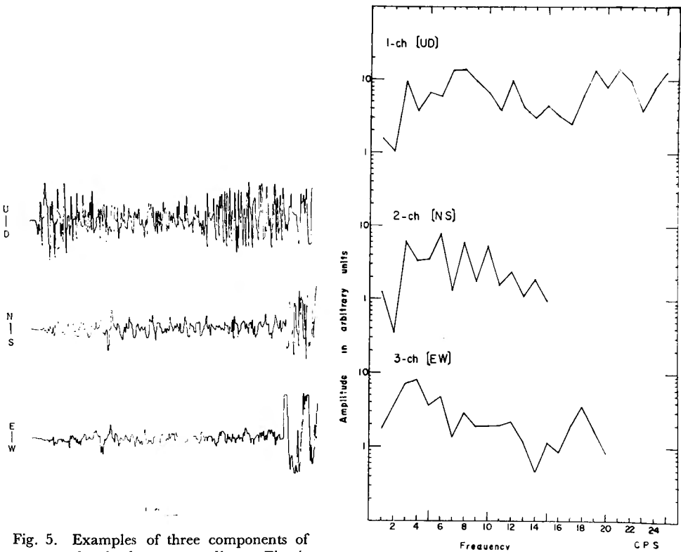
Fig. 6. Examples of Fourier spectrum of p -portion.
