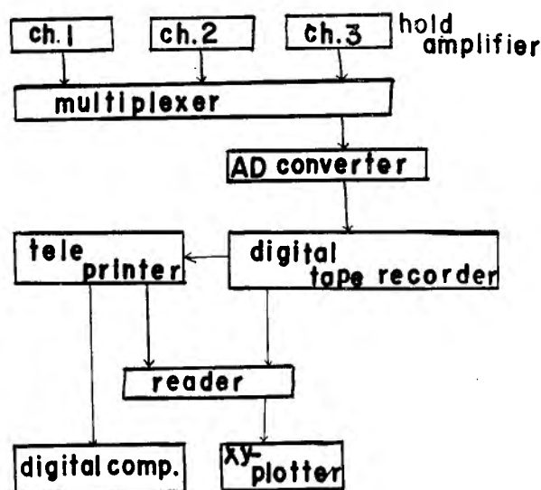
Fig. 1. Block diagram of AD converter.
