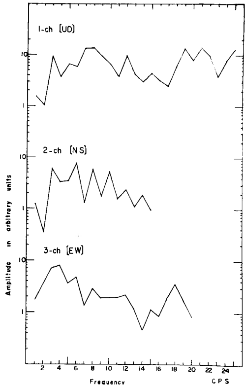
Fig. 6. Examples of Fourier spectrum of p -portion.
