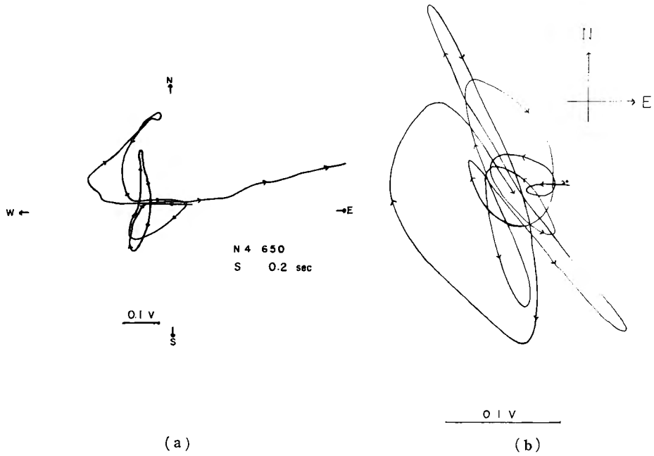
Fig. 4. Examples of wave orbital motions written on XY-plotter from the data sampled with the speed of 1,000 c/s. 4(a) indicates the p -portion and 4(b) the s -portion.
