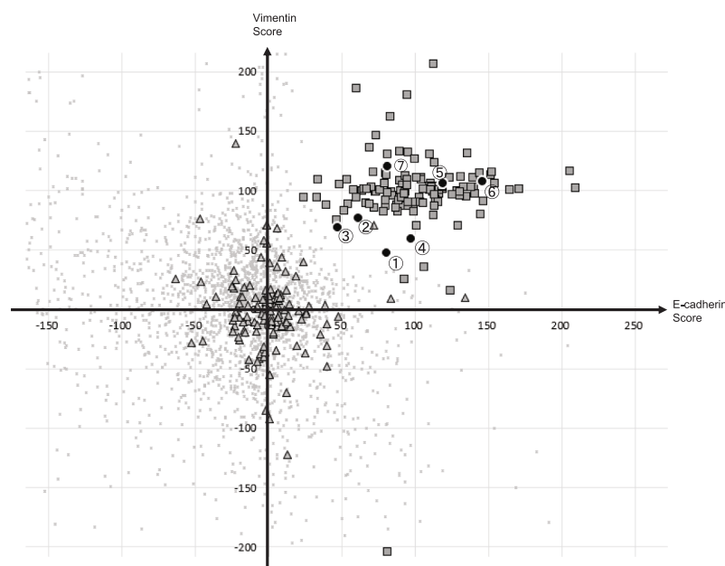
Fig. 3. Compounds screened using NanoLuc-A549 lung cancer cells were scored and plotted. Four compounds and three transforming growth factor-β (TGF-β) inhibitors were identified. Scoring: (\text{Data (DrugX)} - \text{TGF-}\beta\text{1(+)} \text{ Ave.}) / (\text{TGF-}\beta\text{1(-)} \text{ Ave.} - \text{TGF-}\beta\text{1(+)} \text{ Ave.}) \times 100 . Table 1 shows the names, score values, and pharmacological classification of these compounds. ● Compounds identified as hits. × Compounds not identified as hits. ■ Positive control group. ▲ Negative control group.
