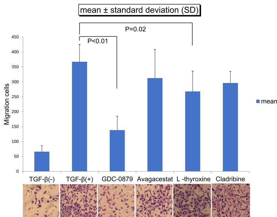
Fig. 6. Matrigel invasion assays were performed to examine the effects of each drug on transforming growth factor-β1 (TGF-β1)-mediated cell invasion. Treatment with GDC-0879 and levothyroxine (L-thyroxine) following exposure to TGF-β1 (1 ng/ml) significantly suppressed the invasive capacity of A549 cells.
