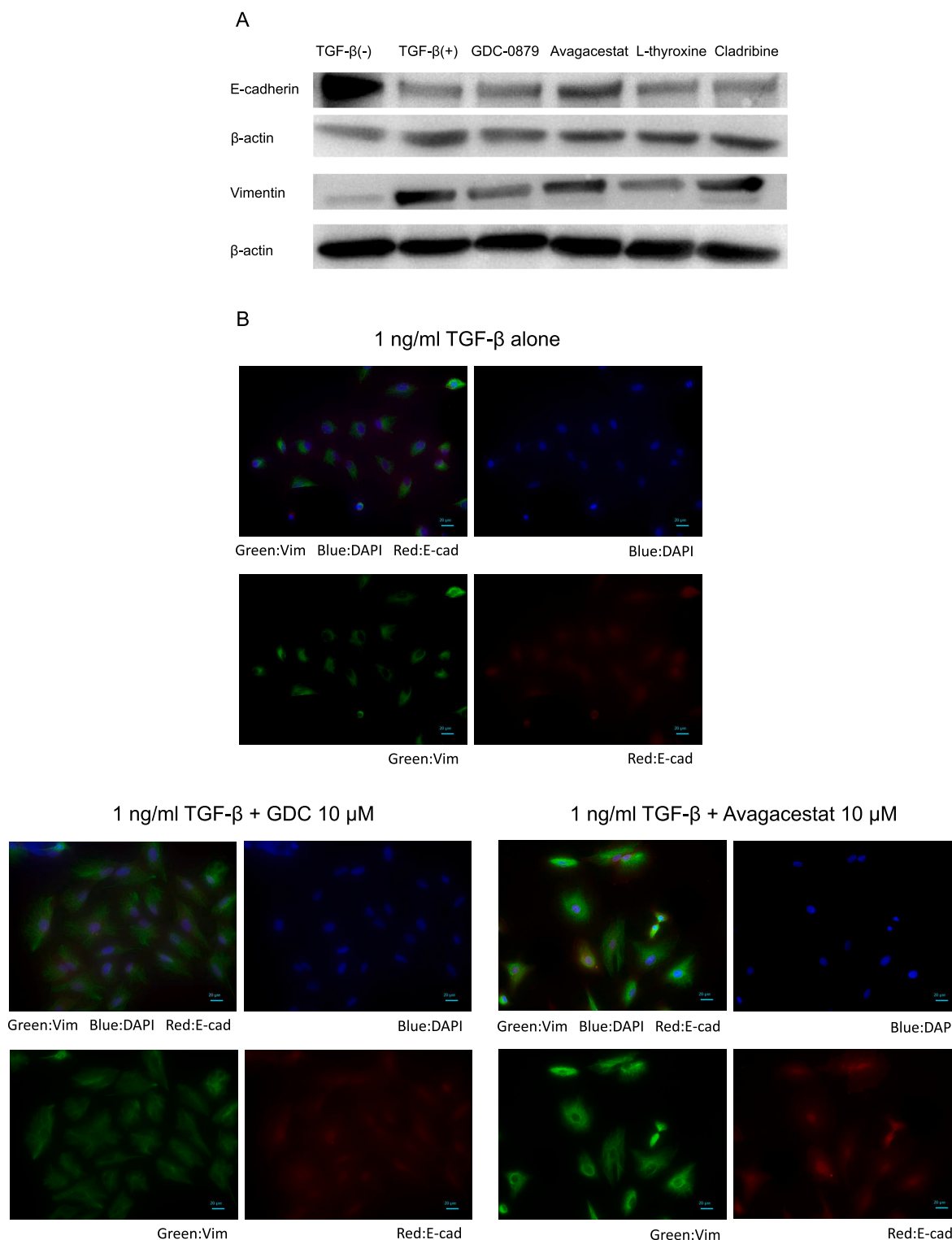
Fig. 4. (A) A549 lung cancer cell lines were cultured for 48 h and pretreated without transforming growth factor- \beta 1 (TGF- \beta 1), with TGF- \beta 1 alone, or with TGF- \beta 1 and each drug (10 \mu M). Cell lysates were immunoblotted to detect the indicated proteins. Avagacestat improved the decrease in E-cadherin expression, while GDC-0879 and levothyroxine (L-thyroxine) improved the increase in vimentin expression. (B) Immunofluorescence image illustrating E-cadherin and vimentin. Alexa 568 (red) staining indicates E-cadherin, Alexa 488 (green) indicates vimentin, and DAPI (4',6-diamidino-2-phenylindole) (blue) indicates the nucleus. Scale bar: 184.52 \mu m. (For interpretation of the references to colour in this figure legend, the reader is referred to the web version of this article.)
