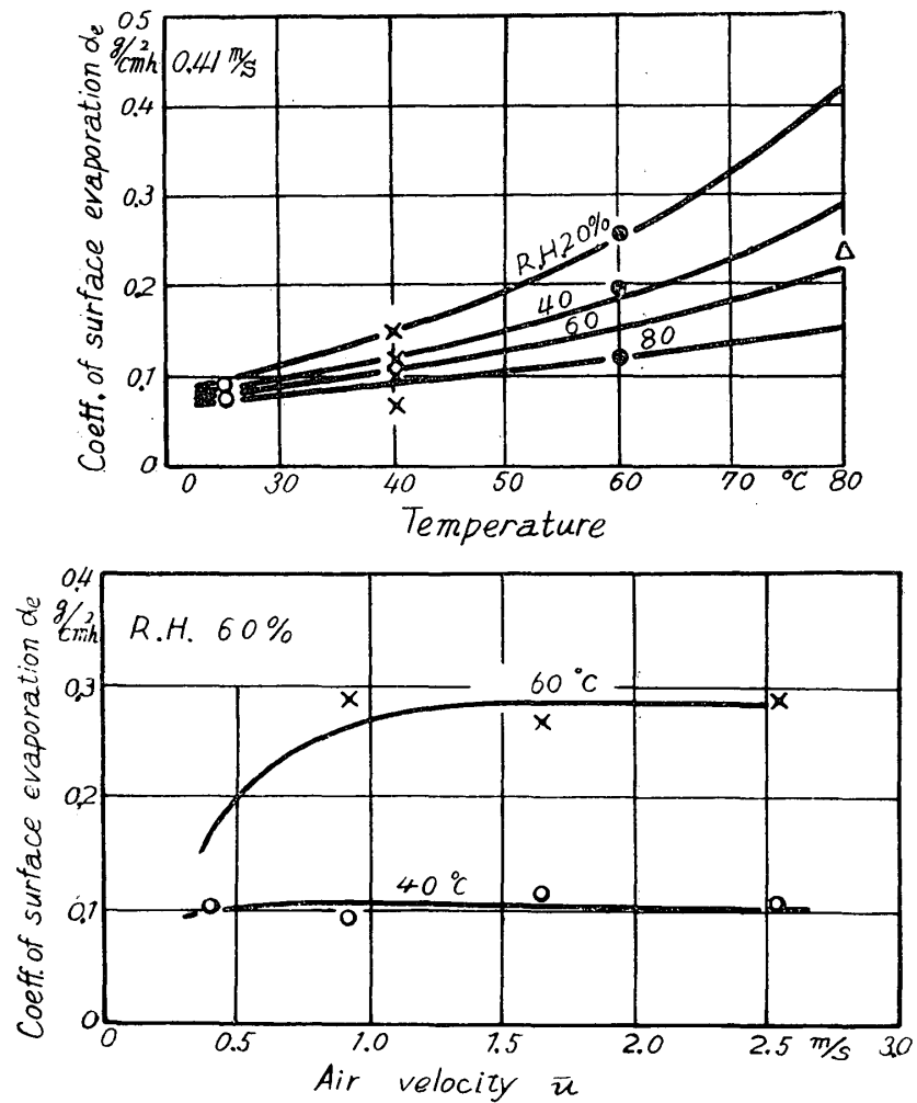
Fig. 26 Relation of longitudinal coefficient of surface evaporation to the drying air conditions ( Fraxinus , for timber of 1.3 cm thick)
