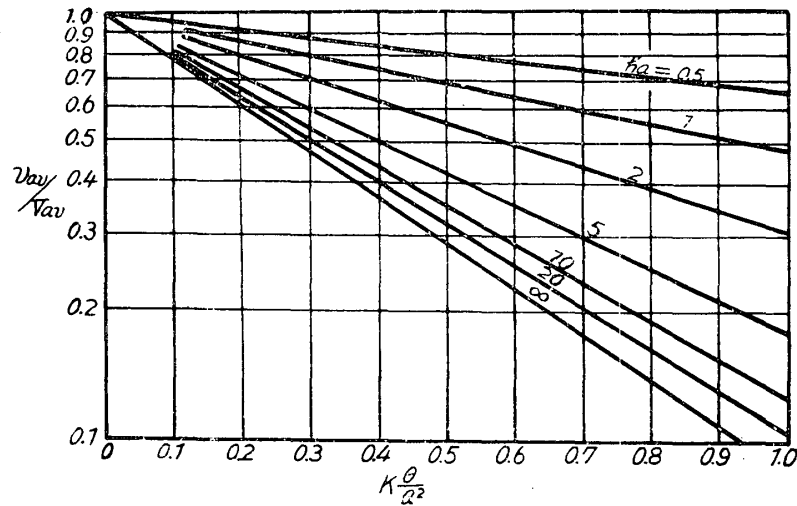
Fig. 4 Dimensionless diagram of eq. (18)
