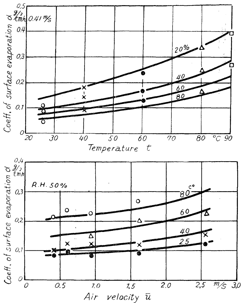
Fig. 34 Relation of transverse coefficient of surface evaporation to the drying conditions ( Fagus , for veneer of 1.5 mm thick)
