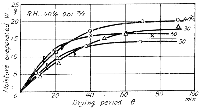
Fig. 31 The curve of the amount of the evaporated moisture ( Shorea , lauaan, 1.24 mm thick veneer)
