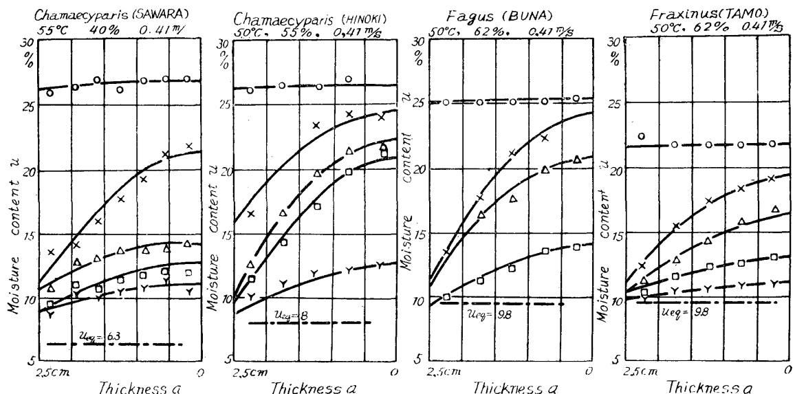
Fig. 23 Gradient of moisture content in longitudinal direction
