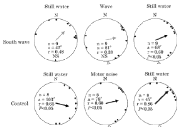
Fig.2 The orientation angle of turtles reared for 0 day to about 2 months in three periods of the wave and motor noise experiments. The dots indicate the mean orientation angle of each turtle. The arrows indicate the mean orientation angle in each group. The length of the arrow represents the intensity ( r ) of orientation in each group. Black arrows represent the turtles significantly oriented, and grays not significantly. White triangles indicate the direction of wave approach or motor noise. NS means “not significant”, and NES means “not enough sample”.
