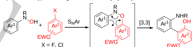
b) Benzidine-type rearrangement of N,O -diarylhydroxylamine
