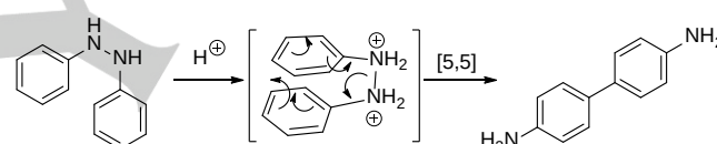
b) Benzidine-type rearrangement of N,O -diarylhydroxylamine
