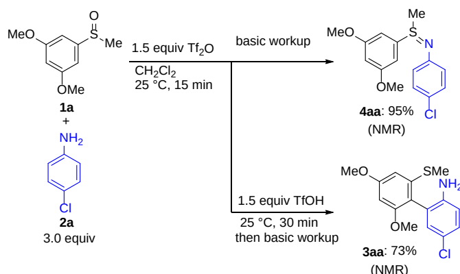
Scheme 2. Initial attempts for dehydrogenative coupling of 1a with 2a
