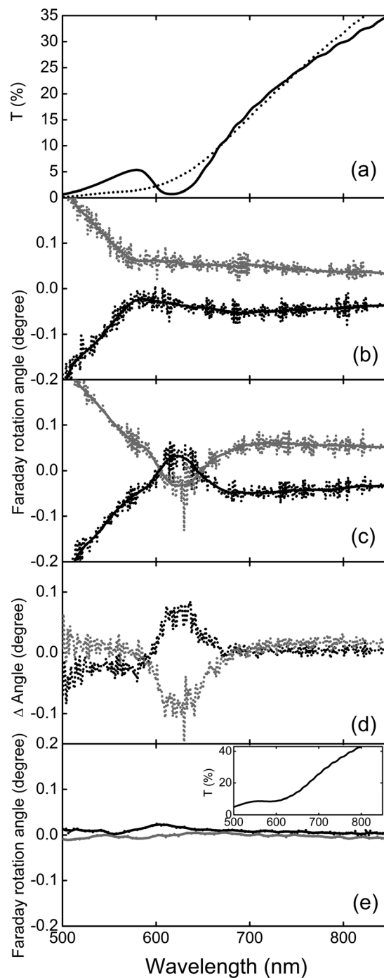
FIG. 2. (a) Optical transmittance of the disordered (a dotted curve) and ordered (a solid curve) domain of the sample. (b) and (c) Faraday rotation of the disordered (b) and ordered (c) domain of the sample. Curves are the guides for the eyes. The black and gray data denote the rotation with the external magnetic field of +15 and -15 kOe, respectively. The data were plotted after subtracting the diamagnetic contribution from a pair of slide glasses sustaining the sample, and also the response of the sample without applying the magnetic field. (d) The difference between the Faraday rotation angle of the ordered domain and that of the disordered domain under the magnetic field of +15 kOe (black) and -15 kOe (gray). (e) Faraday rotation of the reference silica sample consisting of the same silica spheres but without \gamma\text{-Fe}_2\text{O}_3 inside: black ( +15 kOe), gray ( -15 kOe). The data were plotted after subtracting the diamagnetic contribution from a pair of slide glasses and the response of the reference sample under 0 kOe. The inset shows the optical transmittance of the reference sample.
