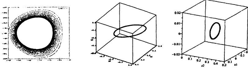
Figure 4: [Left]: Time periodic orbit in (3.7). The horizontal and vertical axes correspond to z_1 and z_2 , respectively. [Middle]: The unstable time periodic orbit in the reduced system (2nd order truncated). Parameters are shown in (3.8). Figure shows the orbit (z_1(t), z_2(t), z_3(t)) , t \in [-3000, -1000] . [Right]: The time periodic orbit around a pure mode solution in third order reduced system. t \in [5000, 6000] .
