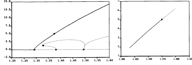
Figure 1: The bifurcation diagram of chemotaxis system(1.7). Coefficients are a = 1/4, d = 16, f = 1, g = p = 1/16 and L = 28.56 . The horizontal and vertical axes correspond to b and \|(u - 1, v - f/g)\|_{L^2} , respectively. Right figure is closeup around a Hopf-bifurcation point on a branch of 2-mode stationary solution.
