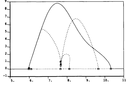
Figure 1: The bifurcation diagram of chemotaxis system(1.7). Coefficients are a = 1/4, d = 16, f = 1, g = p = 1/16 and L = 28.56 . The horizontal and vertical axes correspond to b and \|(u - 1, v - f/g)\|_{L^2} , respectively. Right figure is closeup around a Hopf-bifurcation point on a branch of 2-mode stationary solution.
