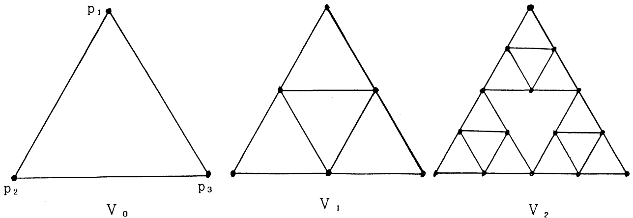
the pre-Sierpinski Spaces for N=3
