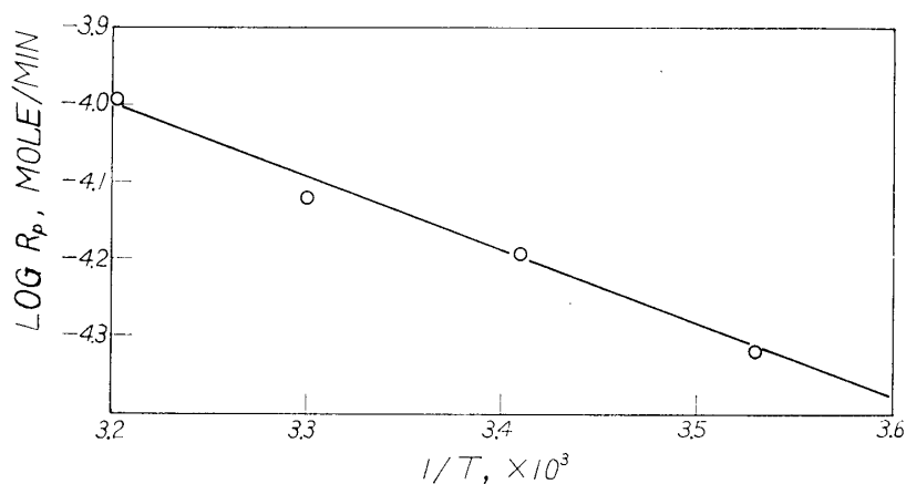
Fig. 10 Arrhenius plot of \log R_p vs. 1/T .
