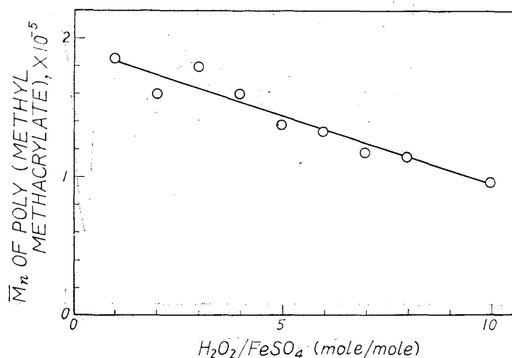
Fig. 7 Number-average molecular weight ( \bar{M}_n ) of branches separated from graft copolymer.
