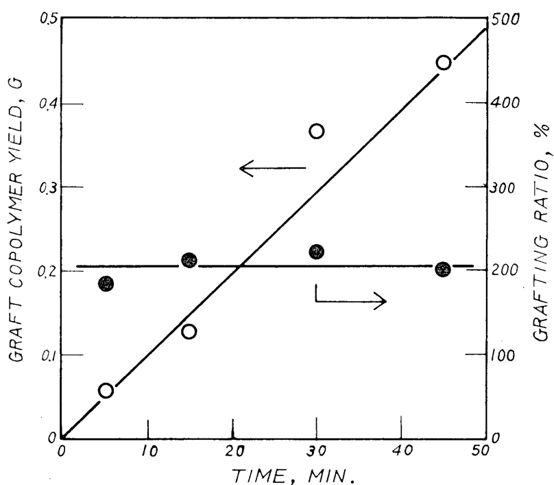
Fig. 9 Relation between graft copolymer yield and grafting time. Grafting conditions: Barium lignosulfonate, 1 g; MMA, 5 ml; [\text{FeSO}_4] = 1 \times 10^{-5} mole/5 ml.; [\text{H}_2\text{O}_2] = 2 \times 10^{-5} mole/5 ml; total volume 15 ml; reaction temperature, 20°C; in vacuo.
