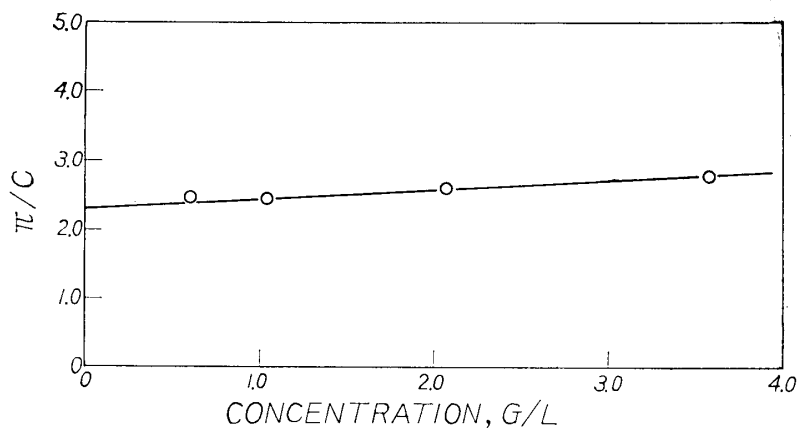
Fig. 1 Relation between osmotic pressure and concentration of dicyclohexylamine salt of lignosulfonate : solvent, water saturated butanol; temperature, 20°C; measured by Melabs membrane osmometer.
