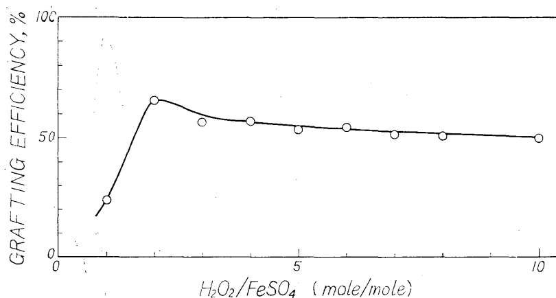
Fig. 6 Relation between ratio of H_2O_2/FeSO_4 and grafting efficiency.
