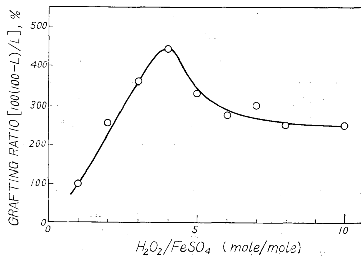
Fig. 5 Relation between ratio of H_2O_2/FeSO_4 and grafting ratio.
