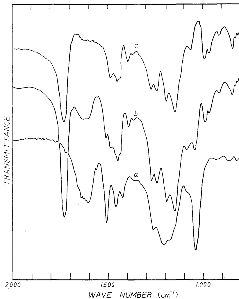
Fig. 4 Infrared spectra of a ; barium lignosulfonate b ; graft copolymer (barium lignosulfonate-methyl methacrylate) c ; poly (methyl methacrylate).
