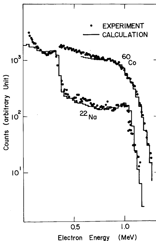
Fig. 3 Examples of stilbene pulse-height spectra obtained for ^{60}\text{Co} and ^{22}\text{Na} gamma rays.
