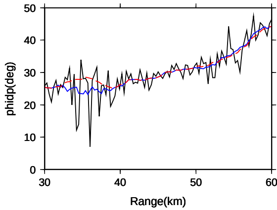
Fig. 10 Observed differential phase \Psi (black line), moving averaged differential phase \phi_{\text{DP}} (blue line) and moving averaged differential phase \phi_{\text{DP}} after filtering (red dash line) in direction of range
