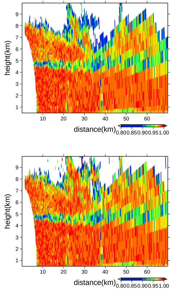
Fig. 9 RHI images of observed correlation coefficient (above) and corrected correlation coefficient (below)
