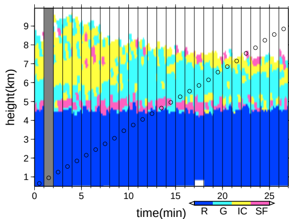
Fig. 16 Hydrometeor classification that used membership function of melting layer height
