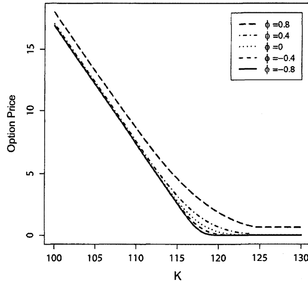
Figure 5: Relationship between K and the option prices for AR(1) process, with \phi = -0.8, -0.4, 0, 0.4 , and 0.8 . We set \kappa = 0.20, \mu = 0.05, r_0 = 0.05 , and \Delta = 1/12 . The option maturity is 1. The bond is 5 year bond with a face value of 100 and a coupon rate of 5%. Coupons are paid semiannually. The parameter \sigma_{AR}^2 is chosen such that the long-run variance \sigma_{AR}^2/(1 - \phi^2) corresponds to 0.01^2 .
