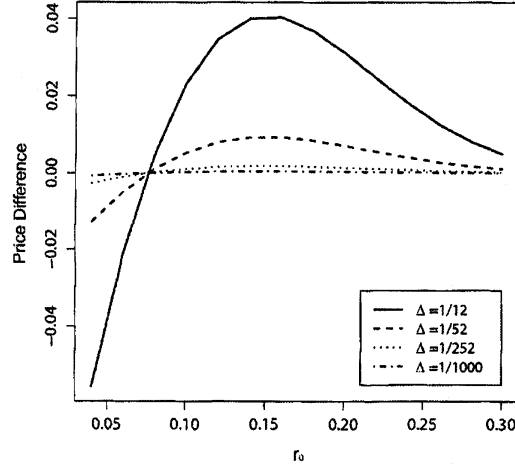
Figure 1: Relationship between r_0 and the option prices differences between the discretized and continuous Vasicek models, with \Delta = 1/12, 1/52, 1/252 , and 1/1000 . Option values are computed for 5 year call on a 15 year 10% coupon bond with a face value of 100. Selected parameter values are \kappa = 0.20 , \mu = 0.085 , and \sigma = 0.02 .
