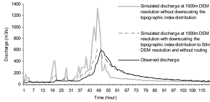
Fig. 10 Comparison of simulation result in Kamishiiba catchment ( 210 \text{ km}^2 ) from scale independent runoff production mechanism. In all the simulation results, 50m DEM resolution TOPMODEL identified parameters are used.
