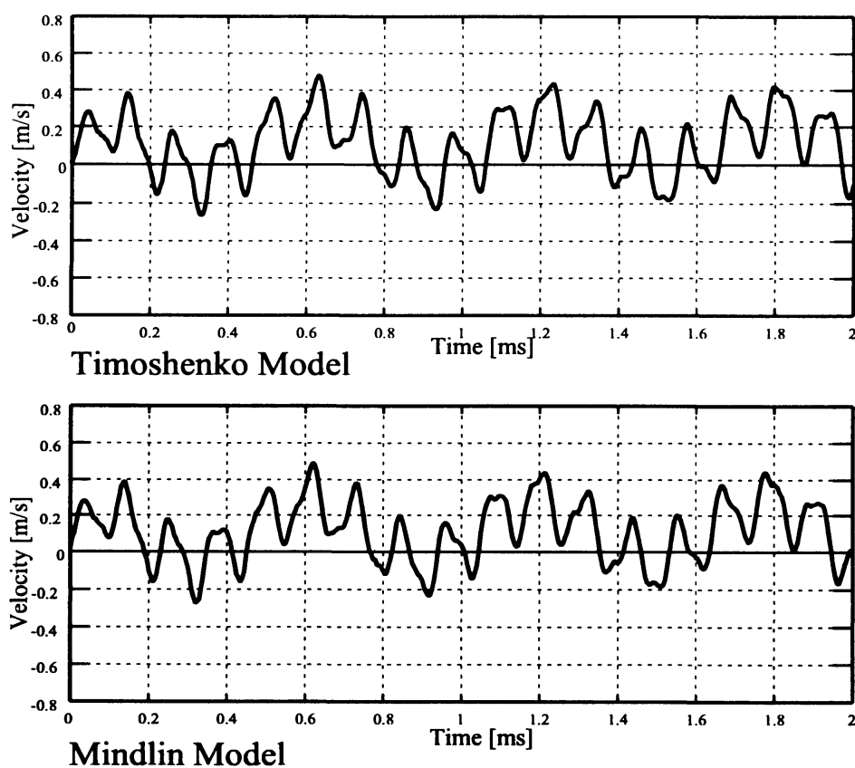
Fig.7. Comparison of temporal waveforms of out-of-plane vibration. The evaluation point is laterally shifted by 5mm from the central line.
