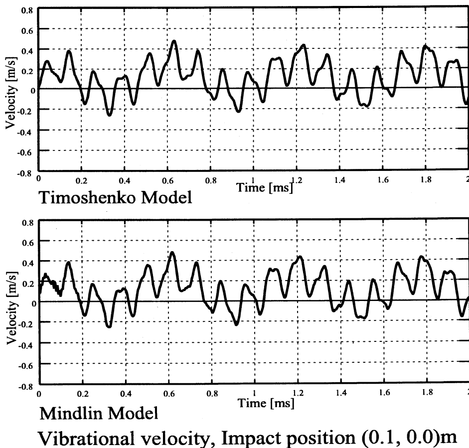
Fig.5. Comparison of temporal waveforms of out-of-plane vibration. The top stands for Timoshenko model and the bottom, Mindlin model. The evaluation point is on the central line.
