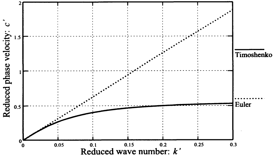
Fig.2 Dispersion Relation
