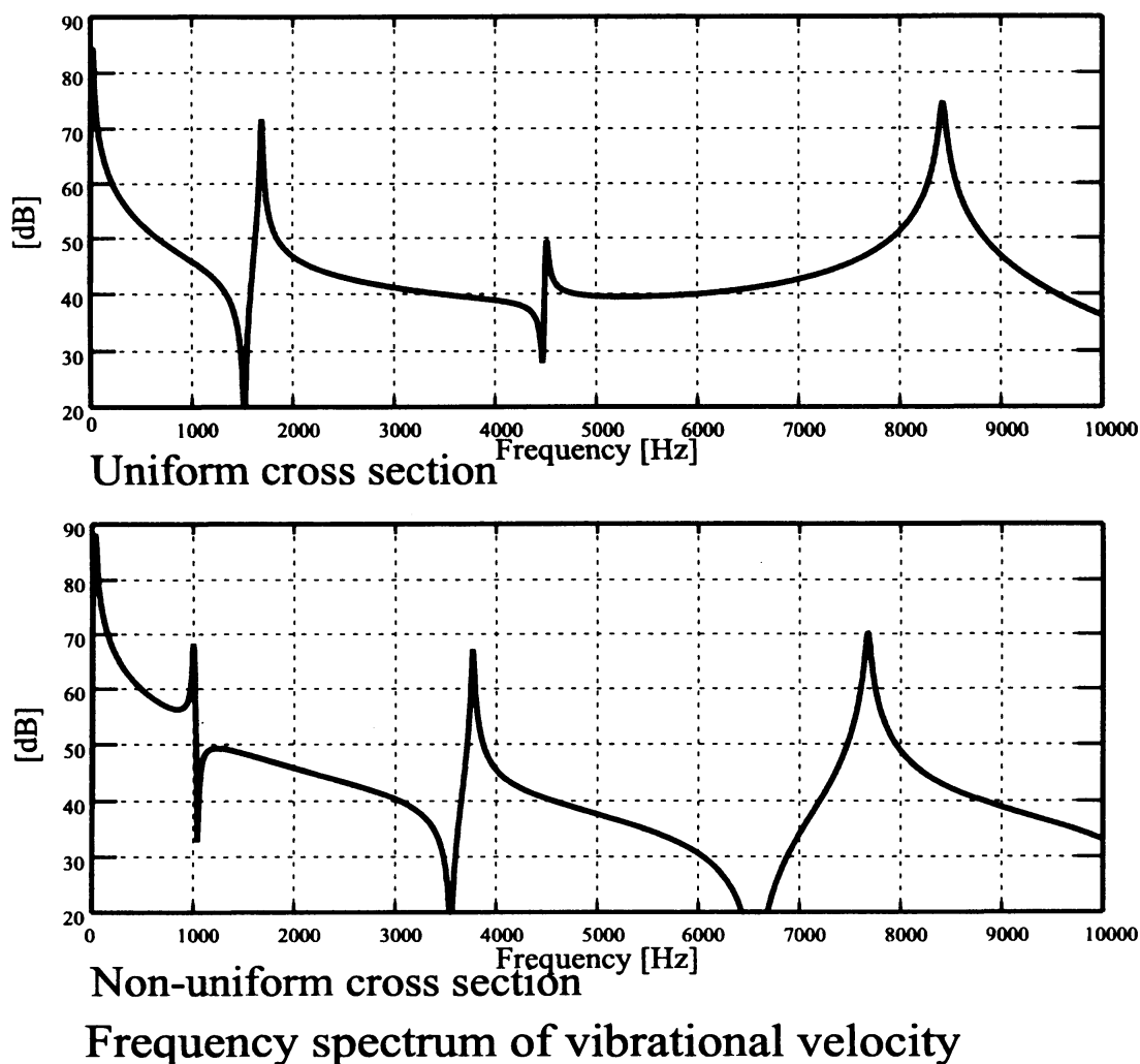
Fig.12. Power spectrums of out-of-plane vibration of the uniform beam (top) and the non-uniform beam (bottom).
