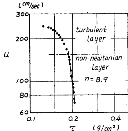
Fig. 3 Velocity distribution
