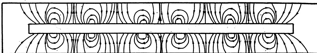
Fig.8 Flow pattern of protons. Since the external boundary condition is taken as a reservoir of n=1.0 , the H^+ flux occurs there.
