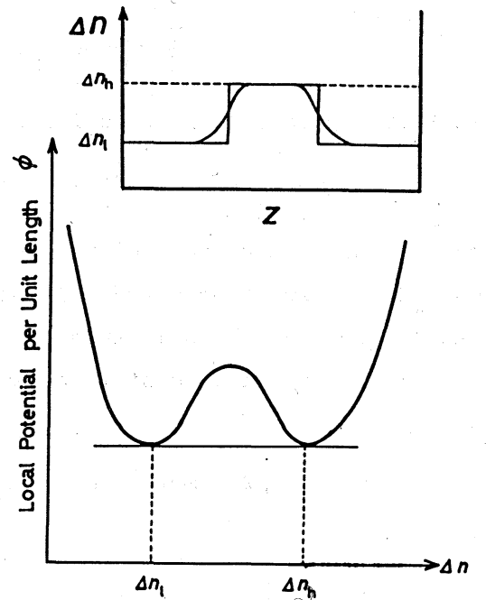
Fig.12 The local potential per unit length for the band-pattern state.
