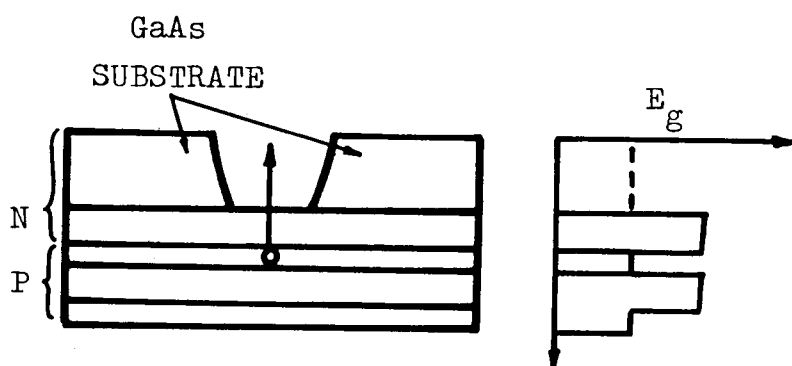
(b) A LED structure with partially dissolved GaAs substrate.
