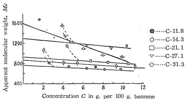
Fig. 3. Plots of Mc versus C for mono-cetyl ether of PEG.
