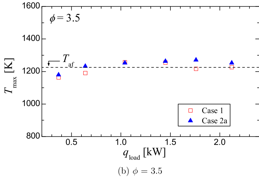
Figure 5.11: Comparison of the maximum flame temperature measured at the axial center of the reactor between Case 1 and Case 2a.
