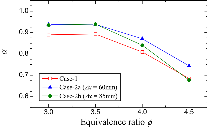
Figure 5.7: Methanol conversion ratio in Case 1, Case 2a, and Case 2b ( q_{\text{load}} = 1.45 \text{ kW} ).
