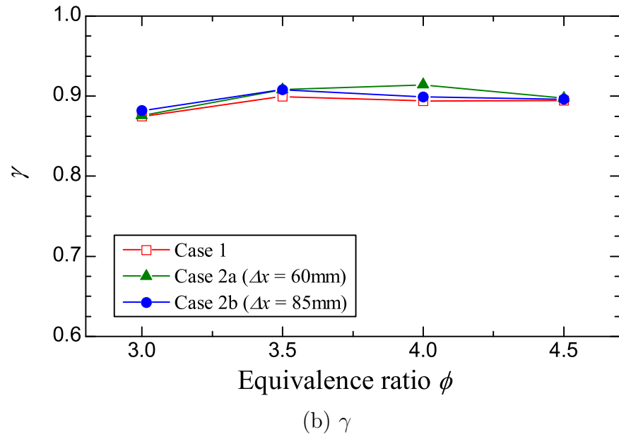
Figure 5.8: Preferential production ratios (Case 1 and Case 2, q_{\text{load}} = 1.45 \text{ kW} ).
