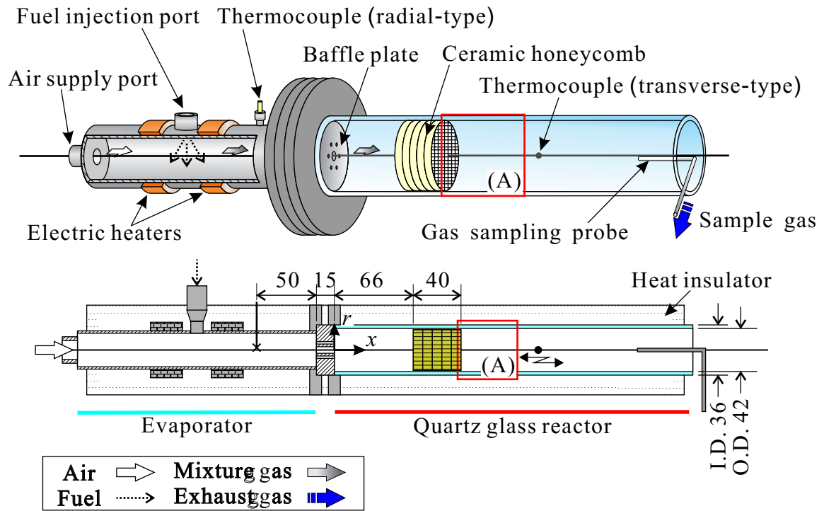
Figure 4.1: Schematic and cross-sectional views of the quartz glass reactor (unit: mm). Square (A) in the figure shows the observation region of the flame in photographs.
