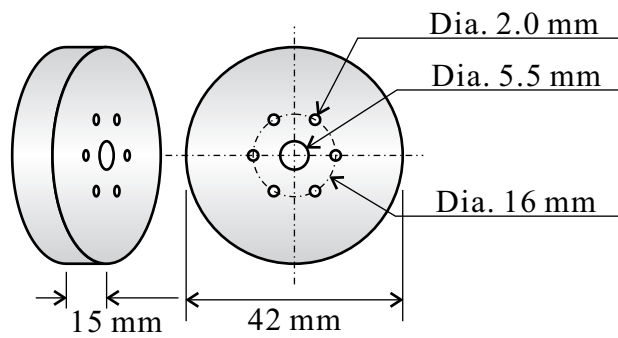
Figure 3.3: Baffle plate.
