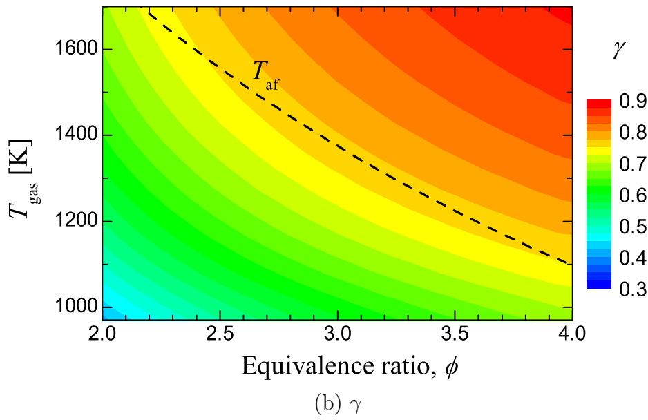
Figure 3.10: Contour of the preferential production ratios with respect to the reaction temperature, T_{\text{gas}} , and equivalence ratio, \phi .
