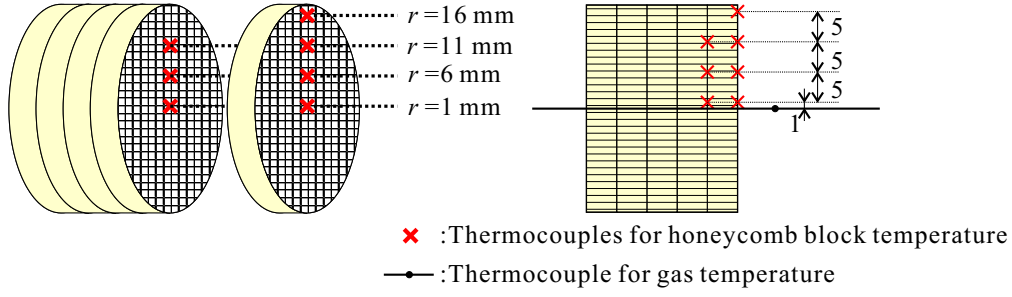
Figure 4.13: Temperature measurement points of the solid surface of the ceramic honeycomb.
