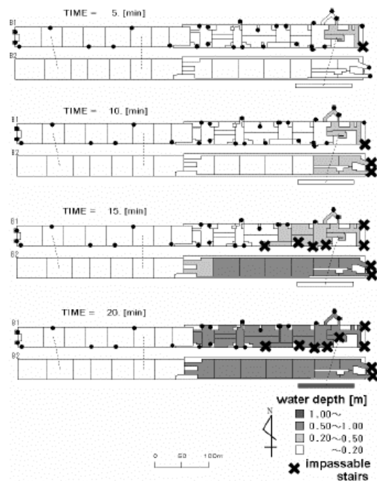
Fig.6 Evacuation possibility
