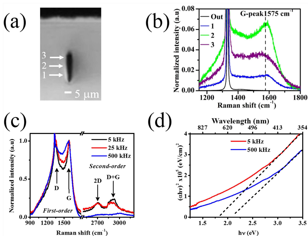
Figure 1. Suppression of graphite in femtosecond laser induced modification at 500-kHz repetition rate.
