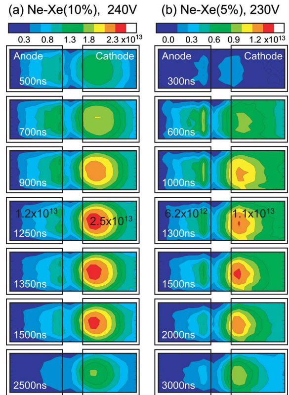
FIG. 6. (Color online) Spatiotemporal behavior of metastable \text{Xe}^*(1s_5) atom density (in units of 10^{13} \text{ cm}^{-3} ) measured in (a) Ne–Xe(10%) panel at the sustain pulse voltage of 240 V and (b) Ne–Xe(5%) panel at a sustain pulse voltage of 230 V in the same situation as in Fig. 5.
