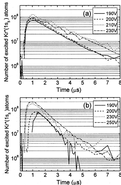
FIG. 9. Temporal behavior of the total number of metastable \text{Kr}^*(1s_5) atoms in the unit cell measured in (a) Ne-Kr(20%) panel and (b) Ne-Kr(40%) panel at several values of the sustain voltage.
