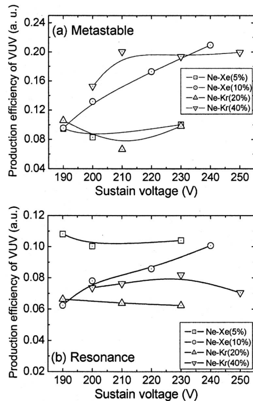
FIG. 14. Production efficiency of VUV photons from (a) metastable atoms and (b) resonance atoms in the four test panels plotted as a function of the sustain pulse voltage.
