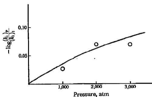
Fig. 8 Plot of \log (k_1)_p/(k_1)_1 vs pressure at 20°C
