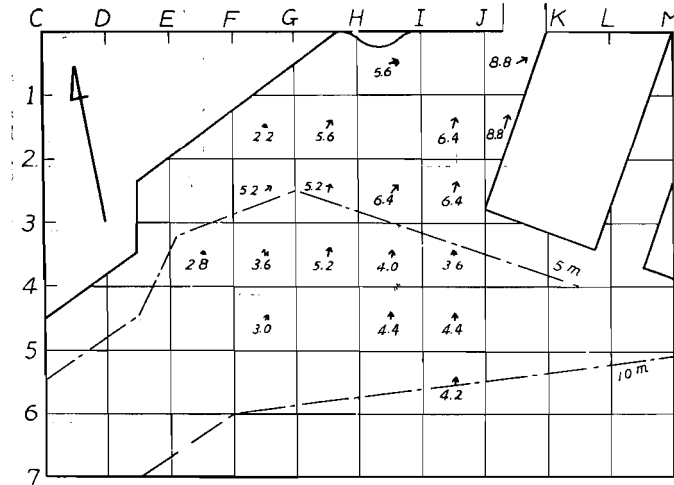
Fig. 10. Pattern of the maximum flood current. Model, x_r/h_r=8 .
