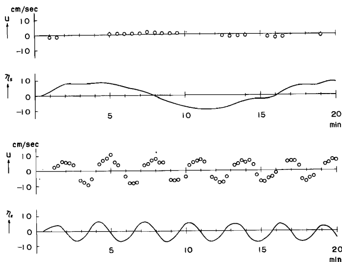
Fig. 41. Velocity of flow u at (A) and water levels \eta_5 at (E) of semidiurnal tide (top) and 130 minutes' oscillation (bottom). Model with the small reservoir.
