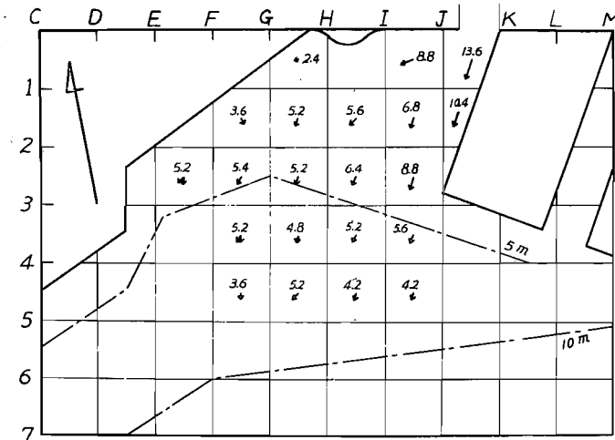
Fig. 11. Pattern of the maximum ebb current. Model, x_r/h_r=8 .
