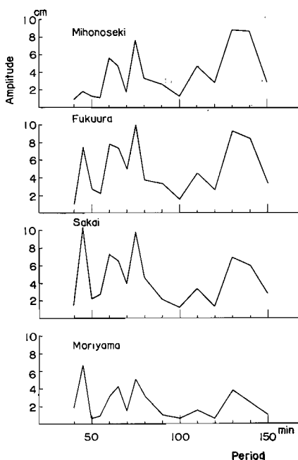
Fig. 22. Periodogram of Chilean Tsunami in Sakai Channel.
