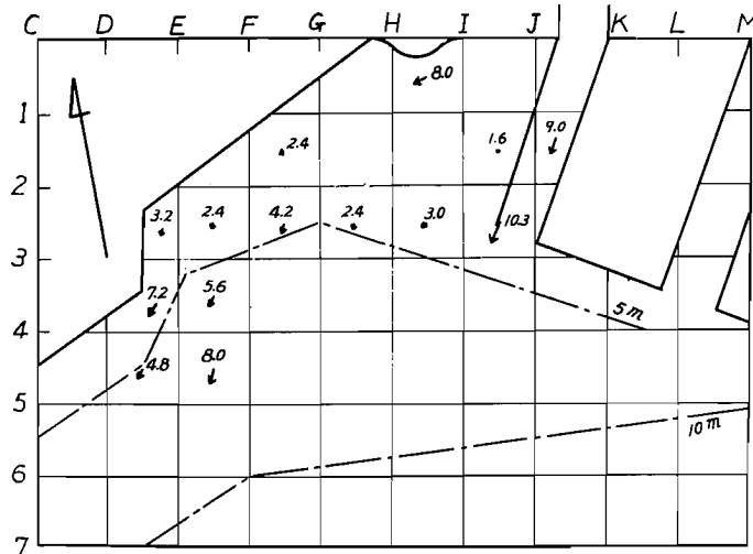
Fig. 16. Effect of the training dyke in the estuary of the Fukushima River. Pattern of the maximum flood current. Model, x_r/h_r=2 .
