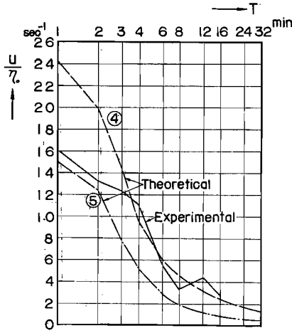
Fig. 62. Velocities of flow of the oscillations of various periods. Experimental and theoretical. Model with the small reservoir.
