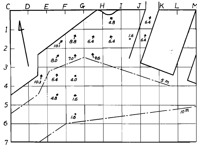
Fig. 17. Effect of the training dyke in the estuary of the Fukushima River. Pattern of the maximum ebb current. Model, x_r/h_r=2 .
