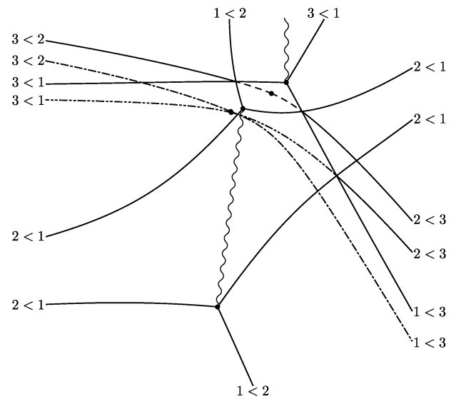
Figure 21. The Stokes geometry of the \text{AKT}_c equation for c = c_{12} .
