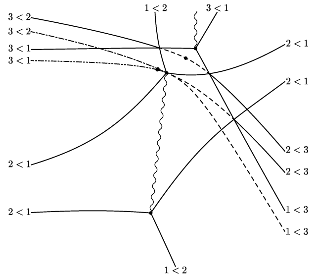
Figure 19. The Stokes geometry of the \text{AKT}_c equation for c = c_{10} .
