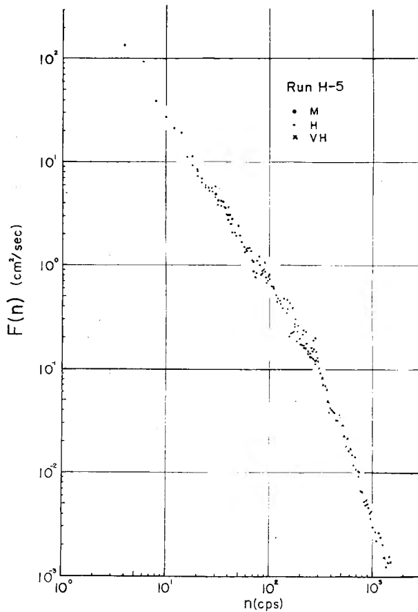
Fig. 6. Energy spectrum of Run H-5.
