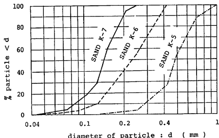
Fig. 1 Particle-size distribution in three types of sand.
