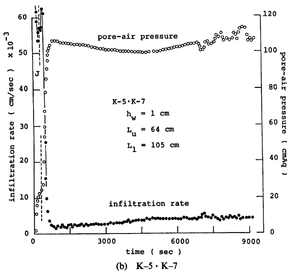
Fig. 2 Changes of infiltration rate and pore-air pressure.
