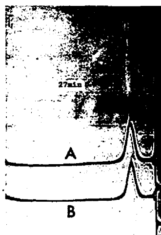
FIG. 3. Sedimentation Patterns of Plant Myrosinase with and without Ascorbic Acid.
