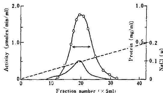
FIG. 3. Chromatogram of Fungous Myrosinase on a DEAE-Sephadex Column (1 x 15 cm).
