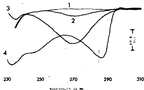
Fig. 4 Differential Spectrum of Myrosinase With and Without ASA.
