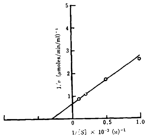
FIG. 7. Reciprocal Plot of Sinigrin Hydrolysis.
