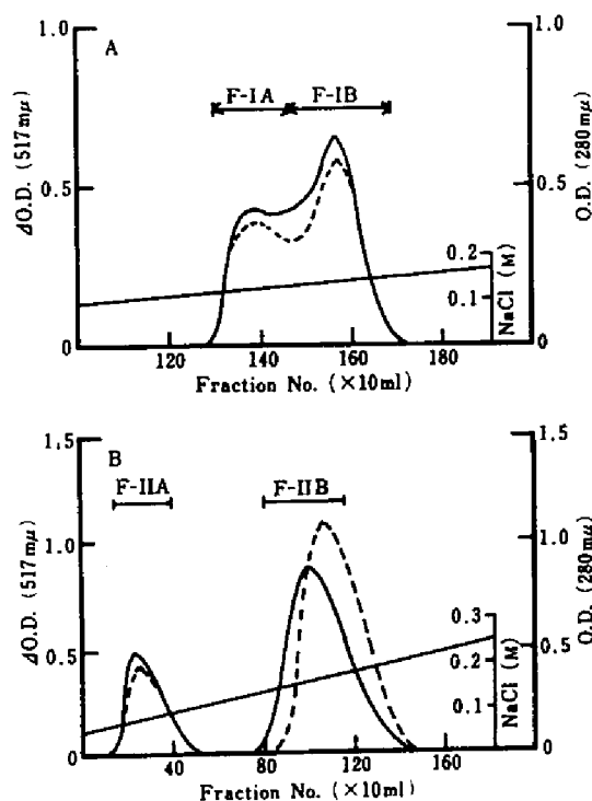
FIG. 3. Chromatography on CM-Sephadex.
