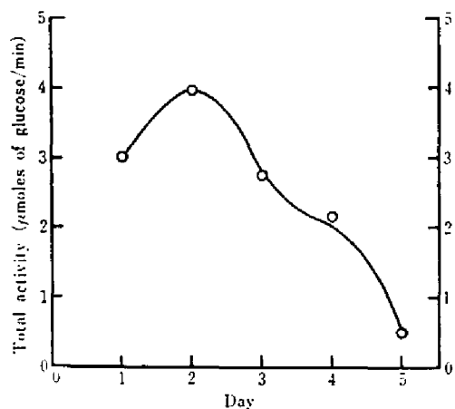
FIG. 1. Enzyme Production in Mycelia of Aspergillus niger .
