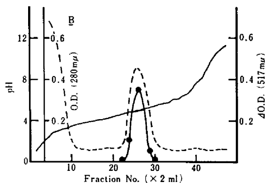
FIG. 9. Isoelectric Focusing of Plant Myrosinases. A; F-IA, B & F-IIA, B; F-IIB.
