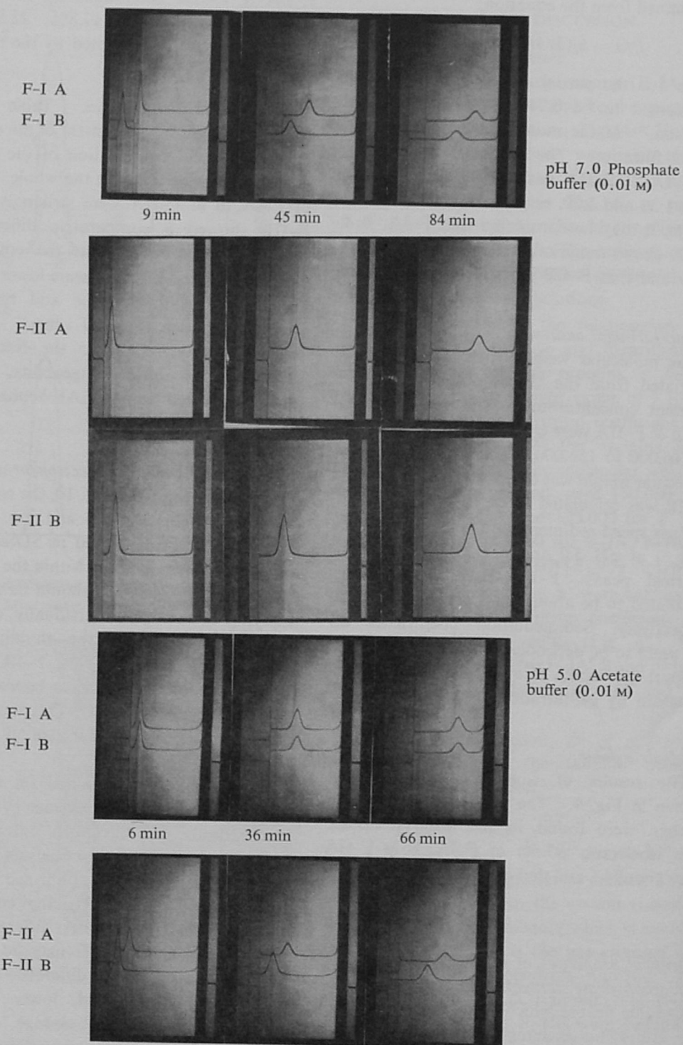
FIG. 6. Sedimentation Patterns of Plant Myrosinases.
