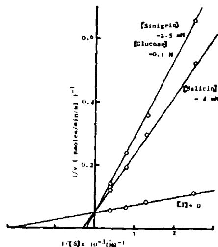
Fig. 11 Inhibitory Effect of Sugar and Glucosides on p-NPG Hydrolysis.
