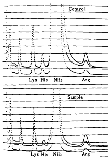
FIG. 8. Comparison of Amino Acid Composition of the Photooxidized and Non-treated Myrosinase.
