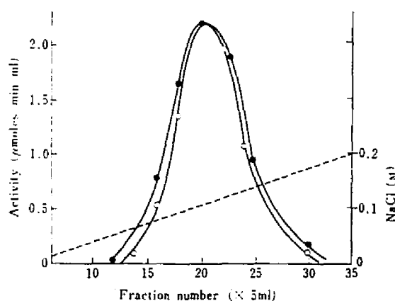
FIG. 8. Chromatogram of the Purified Fungous Myrosinase on a DEAE-Sephadex Column (1 × 15 cm).
