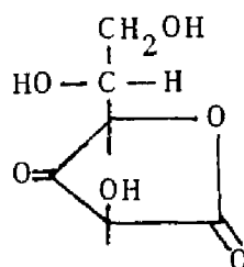
Ascorbic acid (one keto form)
