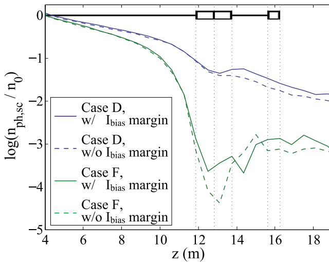
Figure 9. Comparison of one-dimensional profiles of spacecraft-originating photoelectron density between cases with (w/) and without (w/o) the I_{\text{bias}} margin. The blue and green lines correspond to case D ( V_{\text{g-sc}} = -4\phi_{\text{ph}} ) and case F ( V_{\text{g-sc}} = -12\phi_{\text{ph}} ), respectively.
