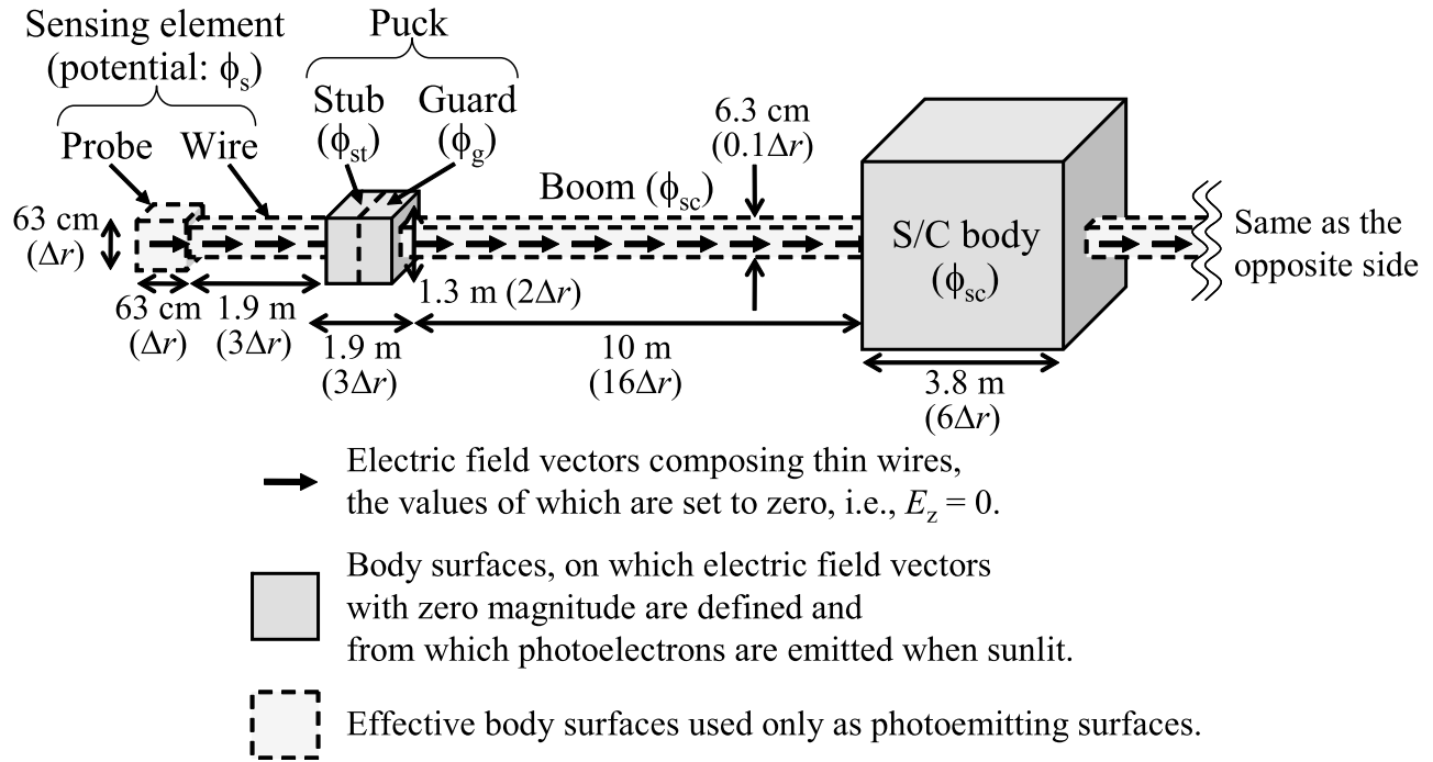
Figure 1. Configuration and dimensions of the numerical model of the electric field sensor used in the present study. Parenthetical symbols (e.g., \phi_s ) displayed below the conducting element names are used for their potentials in the present paper. We define the stub and guard voltages as V_{st-s} = \phi_{st} - \phi_s and V_{g-sc} = \phi_g - \phi_{sc} , respectively. The tip-to-tip length of the sensor corresponds to 52\Delta r .
