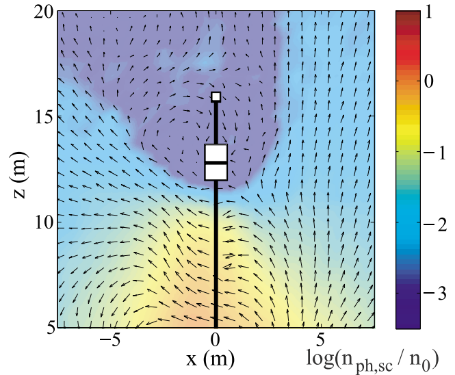
Figure 10. Spacecraft-originating photoelectron flow plotted on a faint color map of the photoelectron density for case F ( V_{\text{g-sc}} = -12\phi_{\text{ph}} ) with the I_{\text{bias}} margin.
