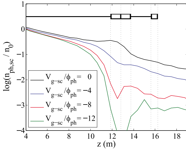
Figure 5. One-dimensional density profiles of the spacecraft-originating photoelectrons measured along an axis (x, y) = (-1.25 \text{ m}, 0) aligned in the z direction and passing through a location adjacent to the sensor.
