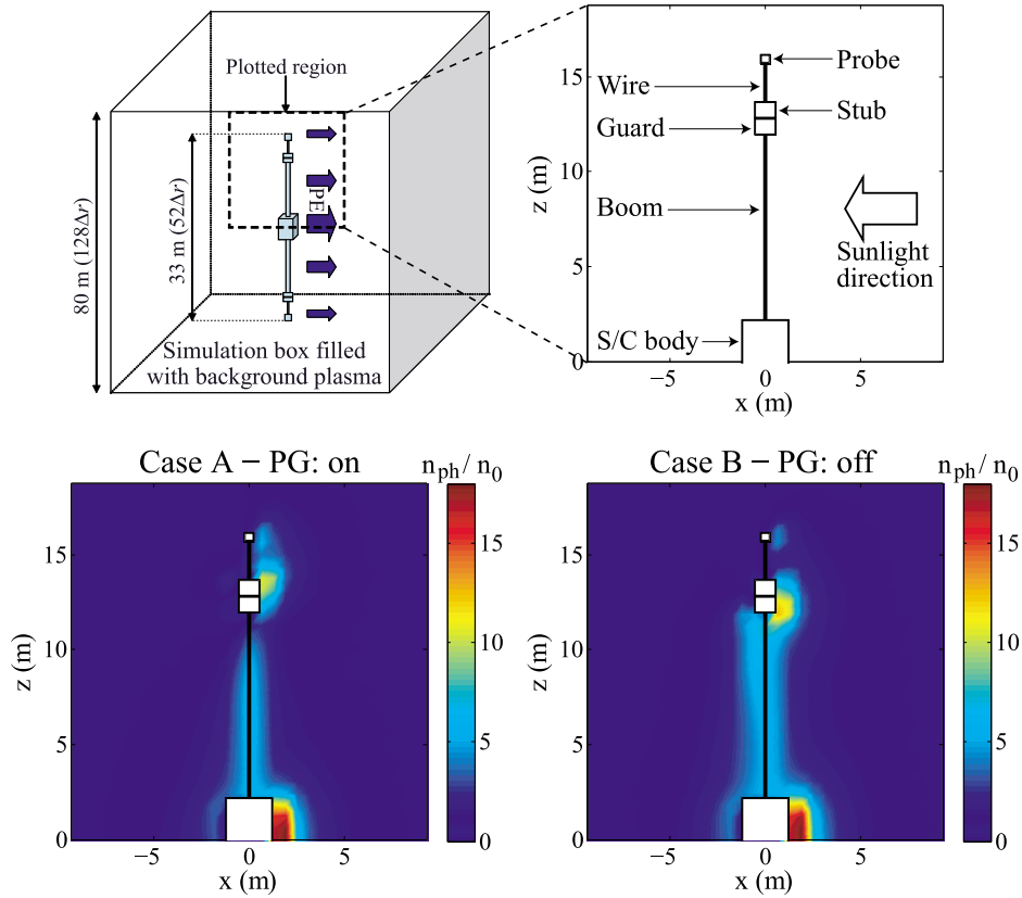
Figure 3. Two-dimensional profiles of the electron density with and without the photoelectron guard (PG) operation on the x - z plane that bisects the center of the spacecraft. (top left) The plotted region in the simulation box. (top right) The sensor and spacecraft positions in the plane. (bottom) Cases of PG: on (case A) and PG: off (case B), respectively. Values are normalized to the background plasma density n_0 .
