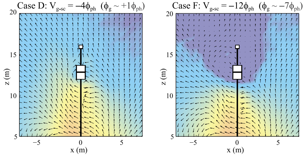
Figure 6. Vector plots of the photoelectron flow for case D ( V_{g-sc} = -4\phi_{ph} ) and case F ( V_{g-sc} = -12\phi_{ph} ). The background color maps show the spacecraft-originating photoelectron density (same as Figure 4).
