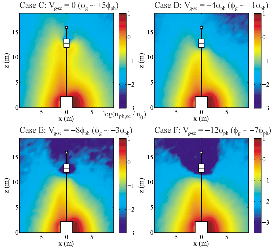
Figure 4. Two-dimensional density profiles of photoelectrons emitted from the spacecraft body measured on a logarithmic scale for case C ( V_{g-sc} = 0 ), case D ( V_{g-sc} = -4\phi_{ph} ), case E ( V_{g-sc} = -8\phi_{ph} ), and case F ( V_{g-sc} = -12\phi_{ph} ). Values are normalized to the background plasma density n_0 .
