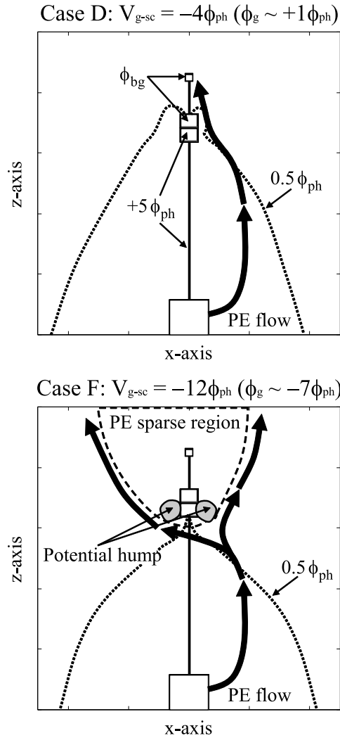
Figure 8. Schematic illustrations of the potential structures influenced by the photoelectron guard electrode and the photoelectron (PE) flow approaching the puck and sensor locations. The dotted lines represent contour lines of potential. The dashed line in case F indicates a photoelectron sparse region created by the photoelectron guard operation.
