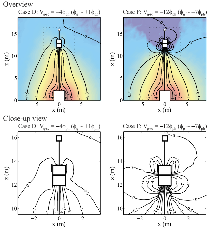
Figure 7. Contour line plots of the electric potential for case D ( V_{g-sc} = -4\phi_{ph} ) and case F ( V_{g-sc} = -12\phi_{ph} ). (top) An overview and (bottom) a close-up view for the vicinity of the puck, respectively. Figure 7 (bottom) focuses on the region that is indicated by dashed line boxes in Figure 7 (top). Potential values are normalized to \phi_{ph} .
