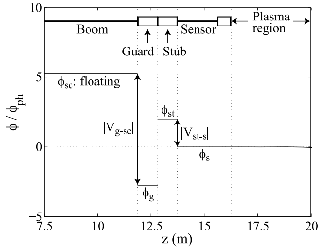
Figure 2. One-dimensional profile of the electric potential along the sensor deployment axis ( z axis). The horizontal axis value represents the distance from the center of the spacecraft. The profile corresponds to the case of the bias current of I_{bias} = -0.75I_{ph0} , where I_{ph0} represents the photoemission current magnitude.
