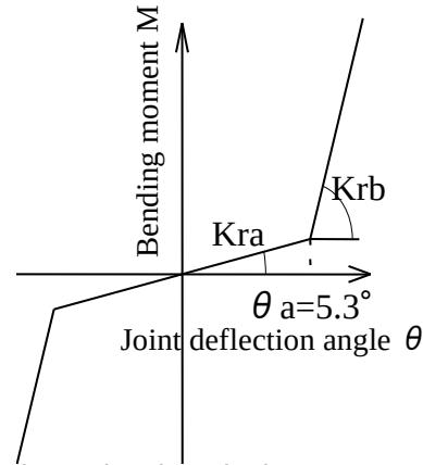
Fig. 4 Joint spring (rotation)
