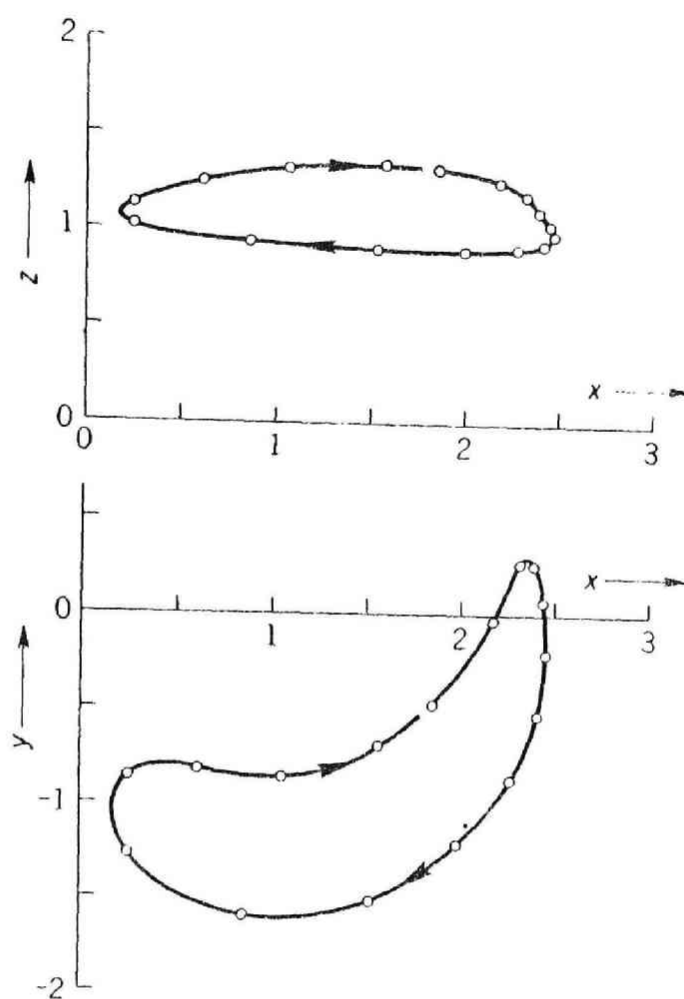
Fig. 5.3 Projections of the limit cycle on the x, y and x, z phase planes. The system parameters are given by Eqs. (5.24).
