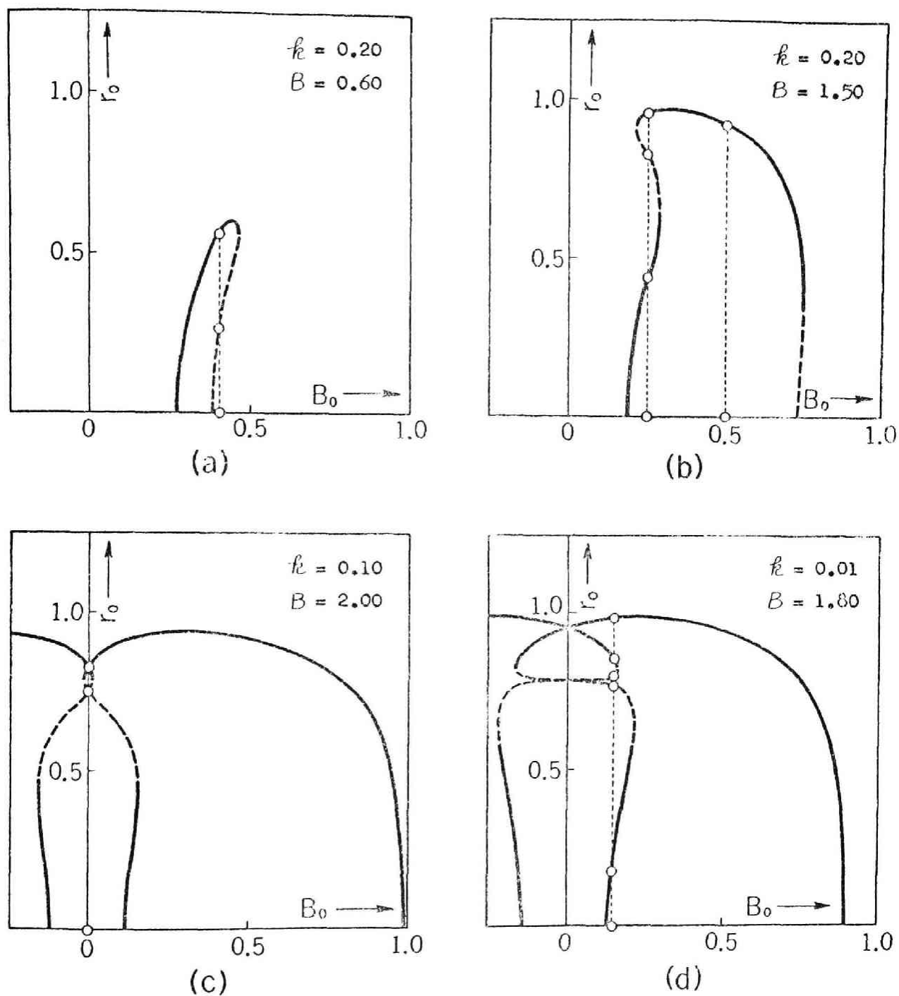
Fig. 3.2 Amplitude characteristics of 1/2-harmonic oscillations.
