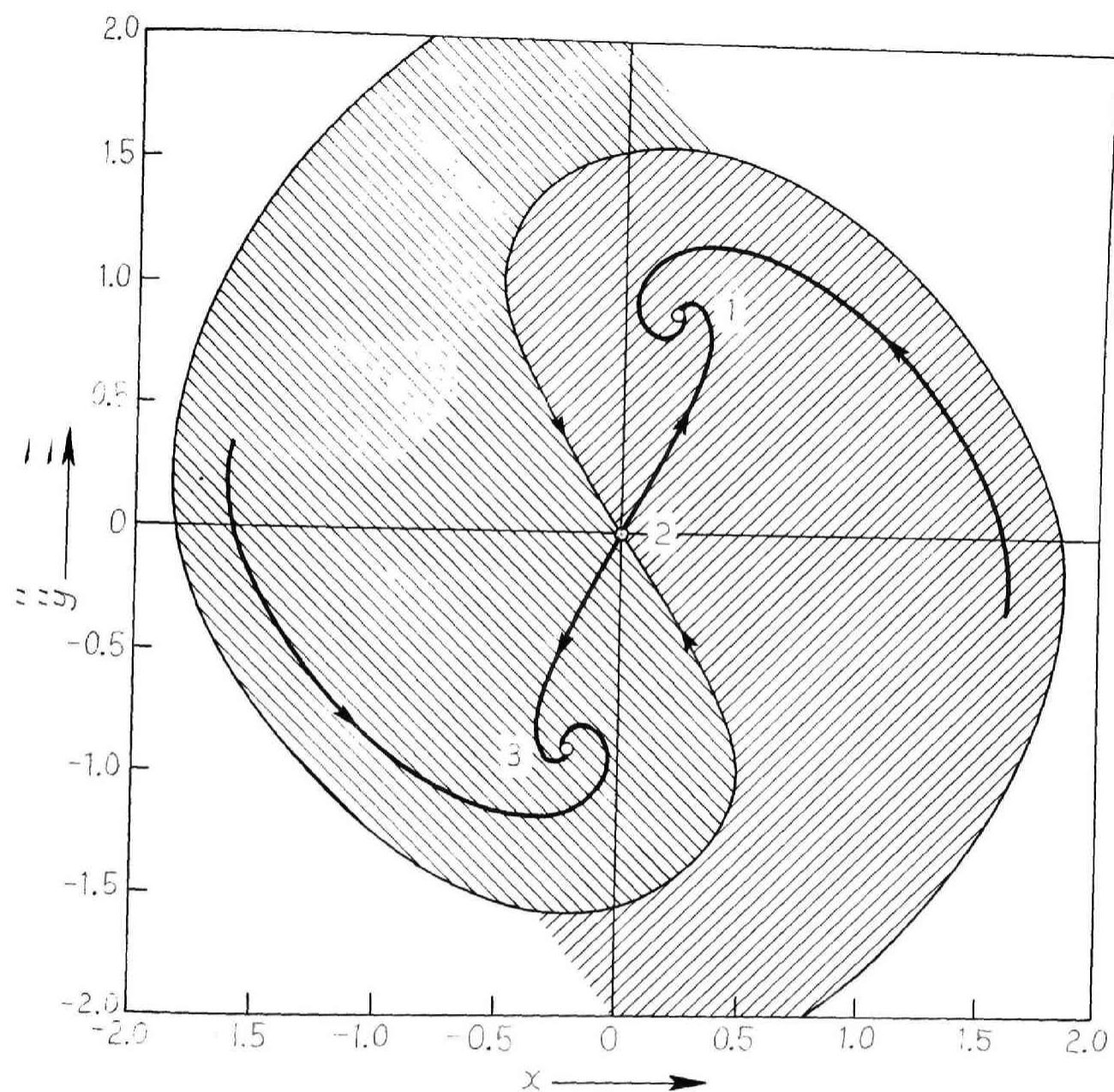
Fig. 3.3 Integral curves of (3.22) in the x, y plane, the system parameters being k=0.20 , B=1.50 , and B_0=0.50 .
