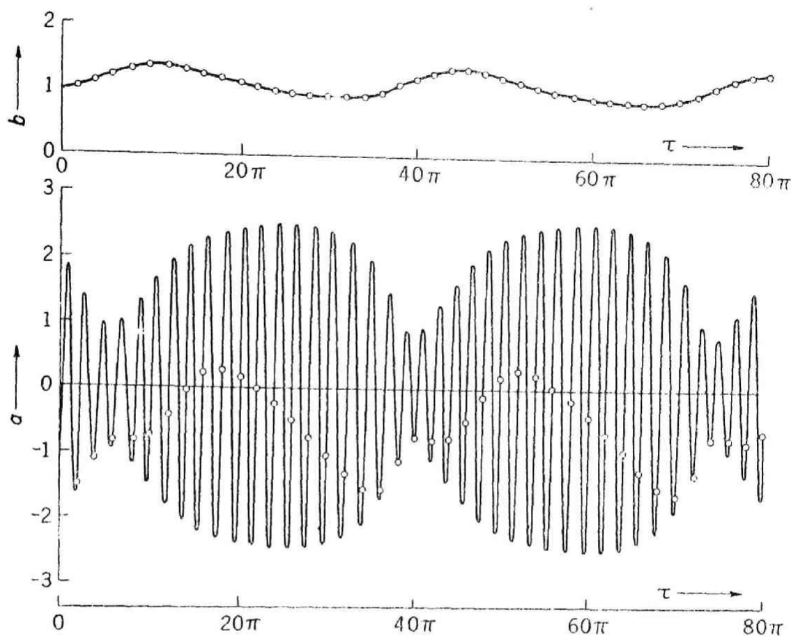
Fig. 5.5 Waveforms of the quasi-periodic oscillation obtained by analog-computer analysis. The system parameters are the same as in the case of Fig. 5.3.
