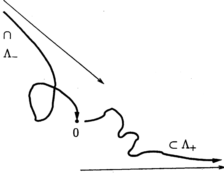
FIGURE 1. The incoming \Lambda_- and outgoing \Lambda_+ Lagrangian submanifolds.
