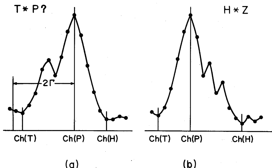
Fig. 5 (a) and (b). Some examples of a deformed peak. (a) The peak may have a sub-peak in lower channels. For this peak, the output printer writes T*P? . (b) The peak has zigzag slope in higher channels. The printer writes the notation H*Z for such a case.
