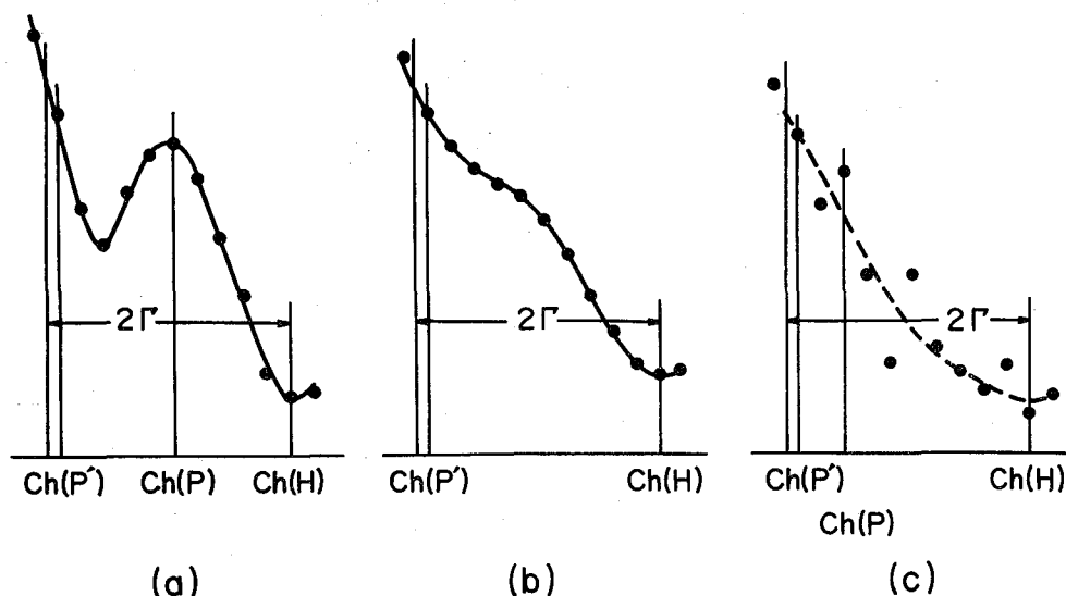
Fig. 3 (a), (b) and (c). Examples of some irregular peaks: (a) a peak having overlapped foot. (b) overlapped and disappeared peak or a peak having larger FWHM than that of standard value. (c) a peak having fluctuation of counts in channels.
