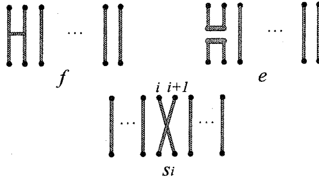
Figure 10: Generators of B
