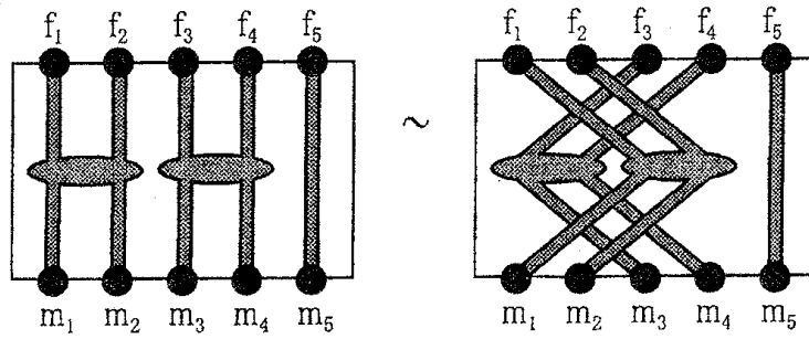
Figure 2: \{\{f_1, f_2, m_1, m_2\}, \{f_3, f_4, m_3, m_4\}, \{f_5, m_5\}\}
