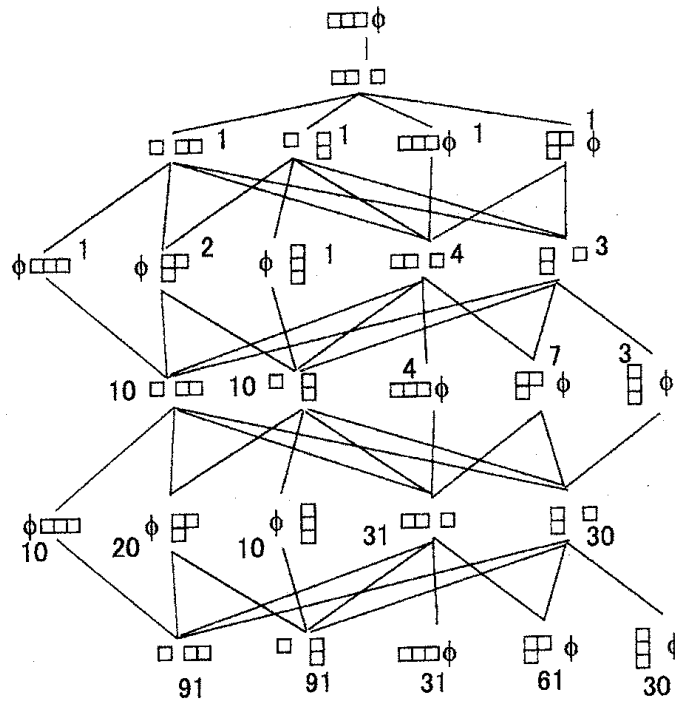
Figure 14: The Bratteli diagram of \text{End}_{G(2,1,3)} V^{\otimes n}
