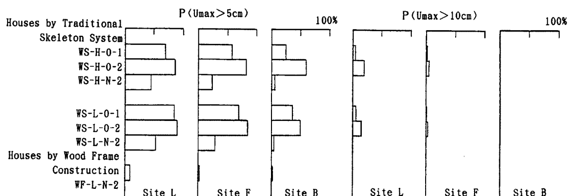
Fig. 11. Comparison of damage ratio in the city of Kyoto during hypothetical earthquake.
