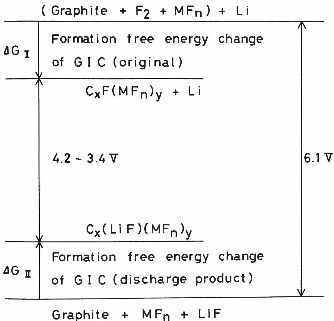
Fig. 4-10 Free energy change in C_xF(MF_n)_y -Li cell.
