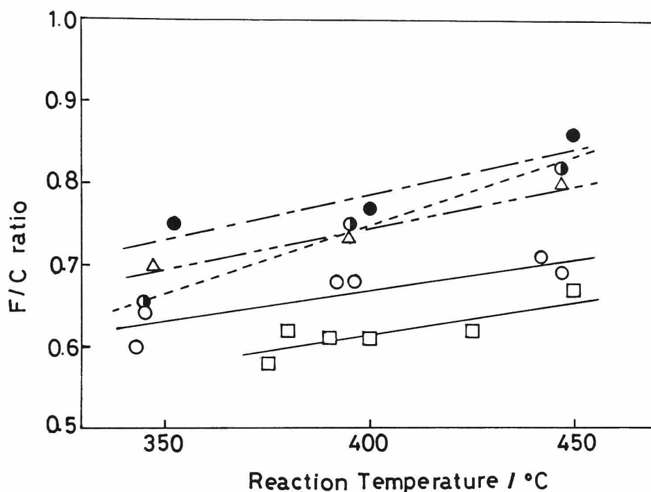
Fig. 5-11 Variation of F/C ratio of graphite fluoride prepared via GIC as a function of reaction temperature.
