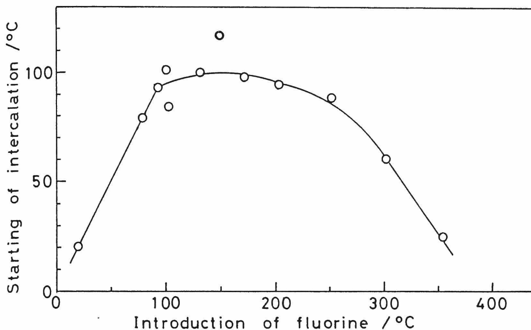
Fig. 2-3 Starting temperature of intercalation vs. the temperature of fluorine introduction.
