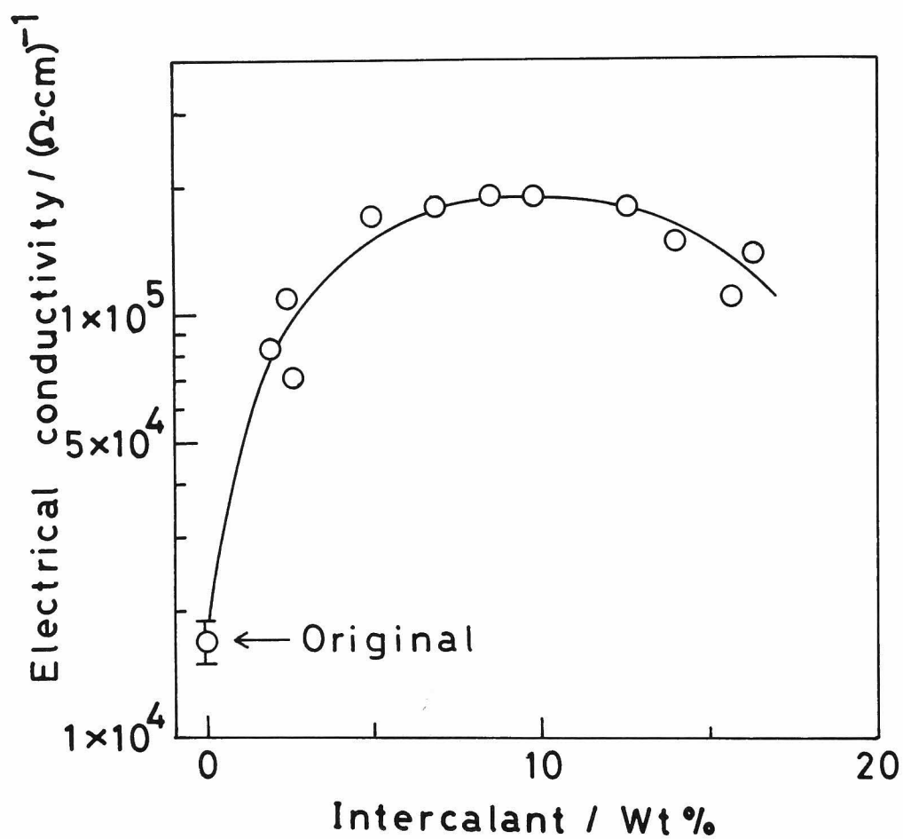
Fig. 3-5 Electrical conductivity ( \sigma_a ) of pyrolytic graphite intercalated by fluorine and \text{MgF}_2 .
