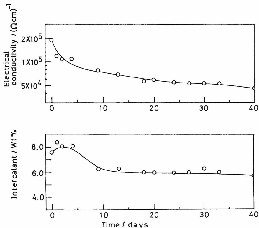
Fig. 3-11 Change in the electrical conductivity and amount of intercalant in air of pyrolytic graphite intercalated by fluorine and LiF.
