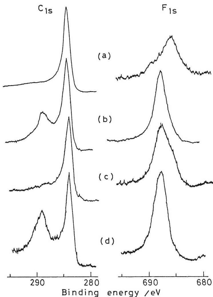
Fig. 1-7 ESCA spectra of C_{x_0}F_y(MgF_2)_y . (a) GIC ( I_c = 9.4 \text{ \AA} ) prepared from PG at 20^\circ\text{C} . (b) C_{7.8}F(MgF_2)_{0.002} prepared from graphitized PC at a retention temp.** of 300^\circ\text{C} for 0.5 h. (c) C_{14}F(MgF_2)_{0.002} prepared from natural graphite at 25^\circ\text{C} . (d) C_{5.5}F(MgF_2)_{0.001} prepared from natural graphite at a retention temp.** of 300^\circ\text{C} for 48 h.
