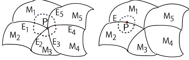
Figure 1: Left: a geodesic circle (dashed curve) with center at an extrinsic vertex p = M_1 \cap \dots \cap M_5 of a piecewise-smooth surface. Right: a geodesic circle (dashed curve) with center at an extrinsic edge point p \in E = M_1 \cap M_2 of a piecewise-smooth surface.
