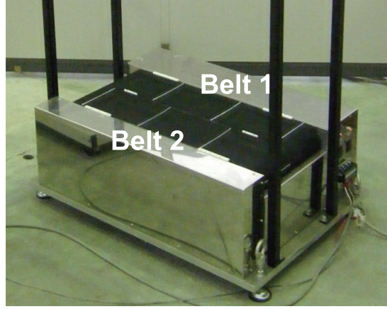
Fig. 3.2: Splitbelt treadmill for the robot.
