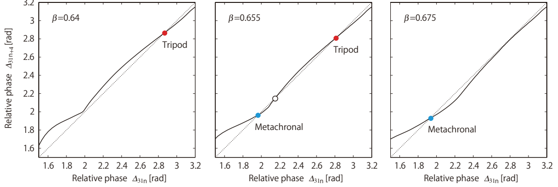
Fig. 2.7: Return maps of the relative phase \Delta_{31} for \beta = 0.64, 0.655 , and 0.675 by plotting the relationship between the relative phase \Delta_{31n} for the n th gait cycle and the relative phase \Delta_{31n} for the (n + 4) th gait cycle. Solid and open dots indicate stable and unstable gaits, respectively.
