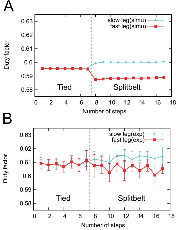
Fig. 4.10: Duty factors of legs for (A) simulation and (B) robot experiments. For robot experiment, data points and error bars are means and standard errors of results of five experiments. Duty factors were identical between legs during tied configuration. They rapidly changed soon after splitbelt configuration started. They remained after rapid change.
