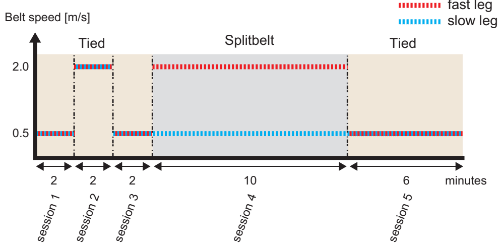
Fig. 4.7: Experimental protocol of human splitbelt treadmill walking composed of five sessions. Session 1 is slow tied configuration for two minutes, session 2 is fast tied configuration for two minutes, session 3 is slow tied configuration for two minutes, session 4 is splitbelt configuration for ten minutes, and session 5 is slow tied configuration for six minutes.
