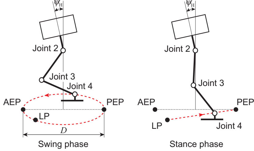
Fig. 3.5: Desired leg kinematics composed of the swing and the stance phases. When the foot lands on the ground, the trajectory changes from the swing to the stance phase. When the foot reaches point PEP, the trajectory moves into the swing phase.
