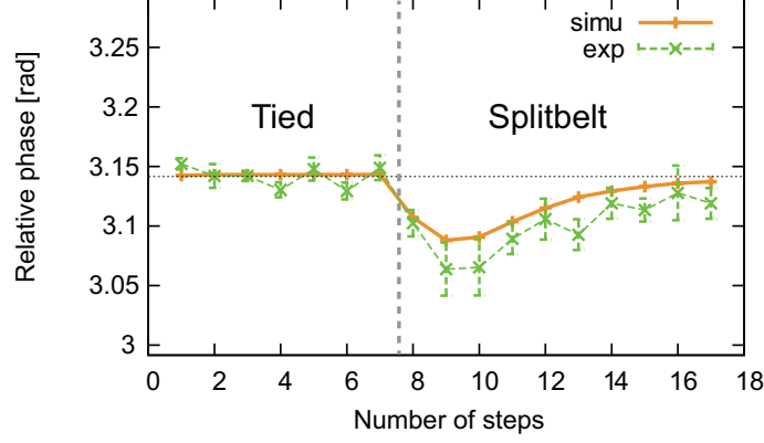
Fig. 4.8: Relative phase between leg oscillators for simulation and robot experiments. For the robot experiment, the data points and error bars are means and standard errors of results of five experiments. During tied configuration, relative phase is anti-phase. Soon after changing to splitbelt configuration, it rapidly shifted. After a while, it gradually returned.
