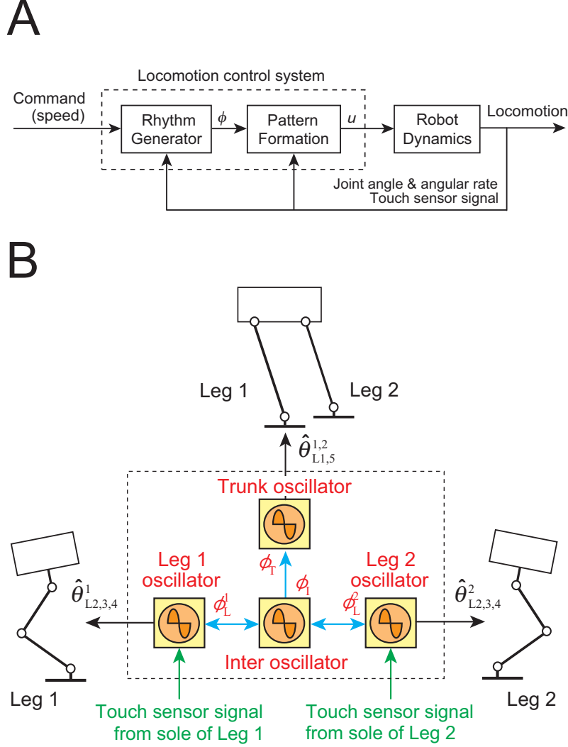
Fig. 3.4: Locomotion control system. (A) Two-layer hierarchical network model composed of a rhythm generator (RG) and pattern formation (PF) models, (B) Phase oscillators for producing locomotor rhythm and motor commands. The blue arrows indicate interactions among the oscillators. The oscillator phases are modulated by phase resetting based on touch sensor signals (green arrows). The oscillator phases determine the leg kinematics (black arrows)
