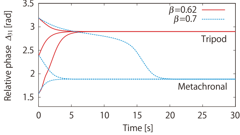
Fig. 2.5: Relative phase \Delta_{31} plotted at contact of leg 1 for three initial values with \beta = 0.62 and 0.7 . For \beta = 0.62 \Delta_{31} converges to 2.9 rad (tripod), while \Delta_{31} converges to 1.9 rad (metachronal) for \beta = 0.7 .
