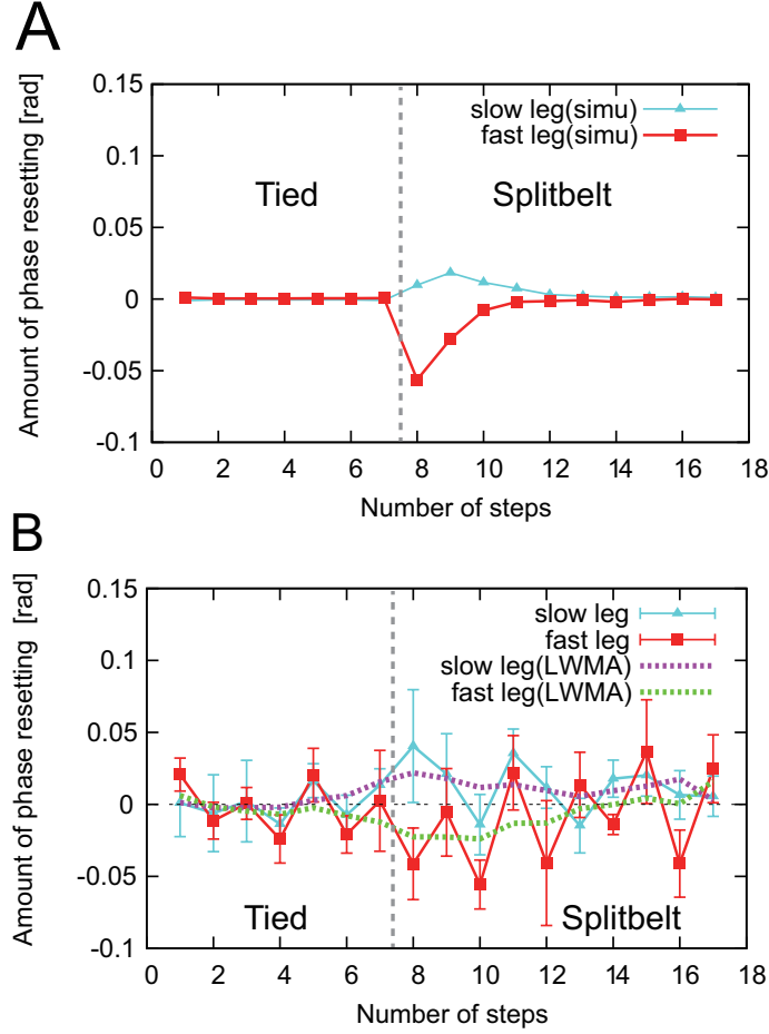
Fig. 4.9: Amount of phase resetting of leg oscillators for (A) simulation and (B) robot experiments. For robot experiment, data points and error bars are means and standard errors of results of five experiments, and dotted lines are five-period linear weighted moving average (LWMA). Amount of resetting was zero during tied configuration, but appeared soon after changing to splitbelt configuration. After a while, it gradually converged to zero again.
