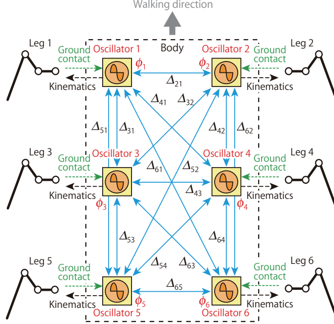
Fig. 2.2: Nervous system model using six oscillators. Solid blue arrows indicate interactions among the oscillators based on the phase relationship \Delta_{ij} . The oscillator phases are modulated by tactile sensor information (dotted green arrows). The oscillator phases determine the leg joint kinematics.
