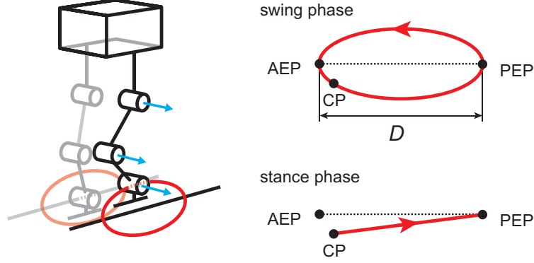
Fig. 4.6: Desired leg kinematics composed of the swing and the stance phases. When foot lands on ground at contact point (CP) (anterior extreme position (AEP) is desired foot contact position), trajectory changes from swing to stance phase. When foot reaches posterior extreme position (PEP), trajectory moves into swing phase.
