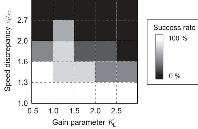
Fig. 3.9: Success rate of splitbelt treadmill walking for various speed conditions and values of K_L . The lower left corner of each box corresponds to the axis value.
