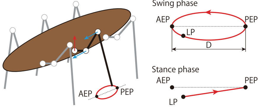
Fig. 2.3: Leg joint kinematics composed of swing and stance phases. The swing phase for the leg tip is a closed curve that includes the anterior extreme position (AEP) and the posterior extreme position (PEP). The stance phase is a straight line from the landing position (LP) to the PEP. When the leg lands on the ground, it changes from the swing to the stance phase. When the leg tip reaches the PEP, it moves into the swing phase.
