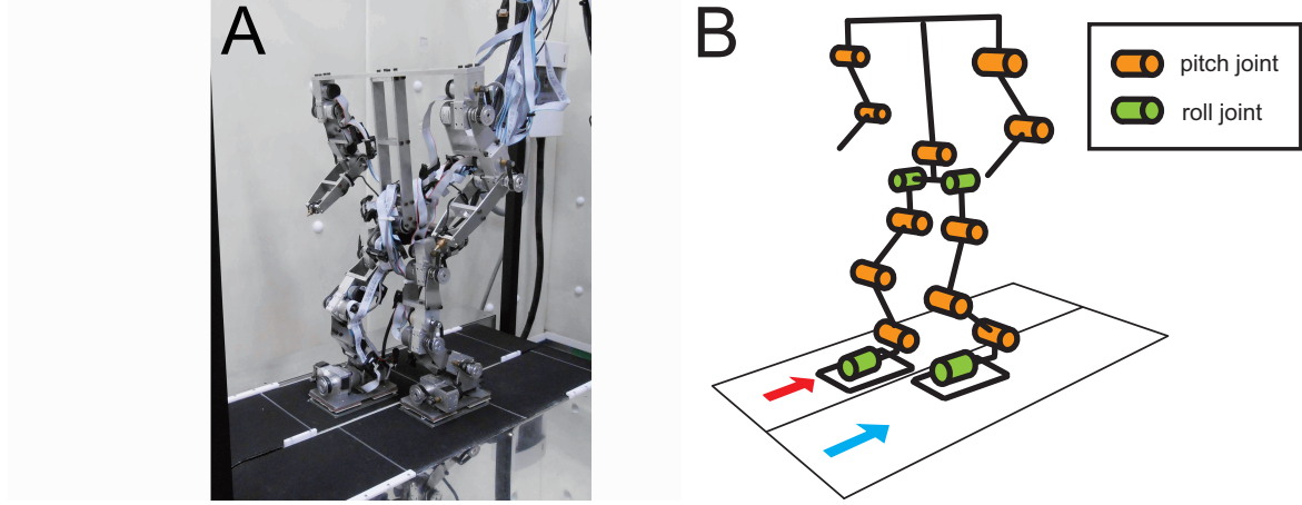
Fig. 4.3: Experimental setup. (A) Biped robot and splitbelt treadmill and (B) schematic model.
