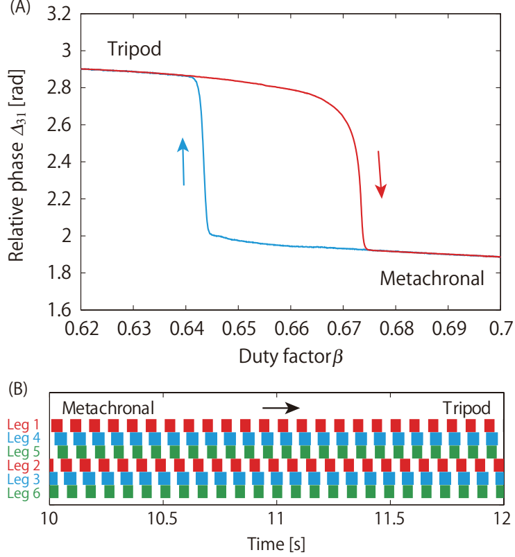
Fig. 2.6: Gait transition induced by changing the locomotion speed through duty factor \beta . (A) Relative phase \Delta_{31} . Metachronal-to-tripod and tripod-to-metachronal gait transitions occur at different locomotion speeds and hysteresis appears. (B) Footprint diagram during metachronal-to-tripod gait transition.
