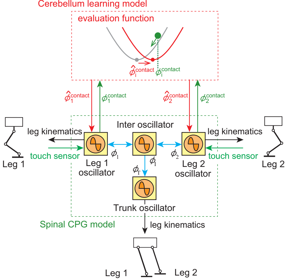
Fig. 4.5: Locomotion control model to show the function of each phase oscillator in spinal CPG model and learning in cerebellar model. Blue arrows indicate interactions among oscillators. Oscillator phases are modulated by phase resetting based on touch sensor signals and desired (predicted) foot contact timing (green arrows). Oscillator phases determine leg kinematics (black arrows). Cerebellar learning model receives phase information at foot contact (green arrows) and modifies desired (predicted) foot contact timing using evaluation function, which is sent to spinal CPG model (red arrows).
