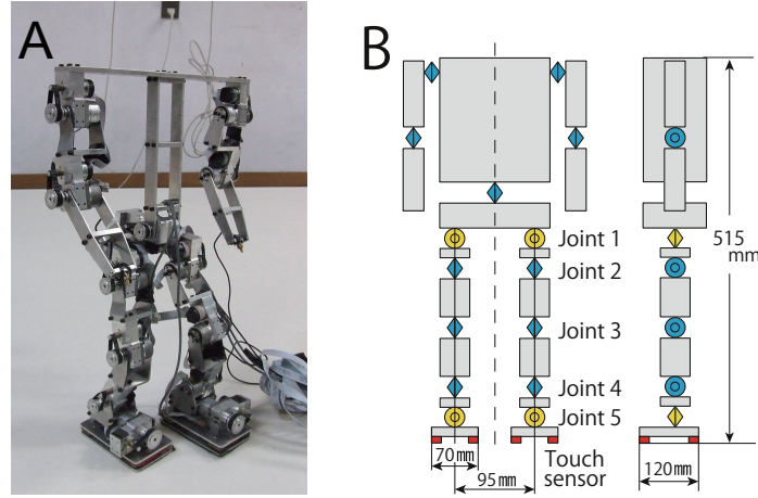
Fig. 3.1: (A) Biped robot, (B) Schematic model of the robot
