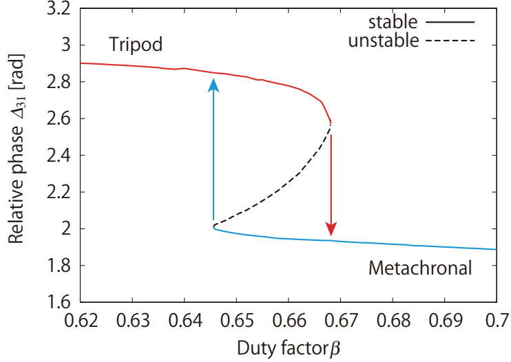
Fig. 2.8: Stable and unstable gaits calculated from the return maps. Two stable gaits and one unstable gait coexist from \beta = 0.645 to 0.67 . Fold catastrophe occurs at connections of the stable and unstable gaits and induces jump of gaits.
