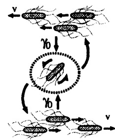
図 1: 1d model
