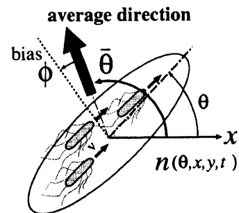
図 5: 2d model
