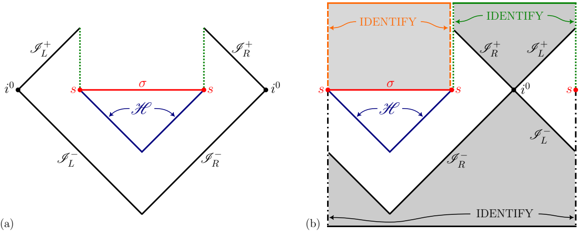
FIG. 3. A full conformal diagram describing the formation and evaporation of a 1+1 Schwarzschild-like black hole (a), accompanied by an illustration demonstrating a conformal embedding of the 1+1 evaporating black hole in a region of the 1+1 trousers spacetime (b). In the 1+1 case, the respective future and past null infinity \mathcal{I}^+ and \mathcal{I}^- are split into two distinct lines distinguished by the subscripts L and R . The lines labeled \mathcal{H} represent the horizon and \sigma represents the classical singularity, which we suppose is regularized by quantum gravity effects. In (b), the dotted lines are identified, as are the points labeled s and i^0 , which are the evaporation point and spatial infinity, respectively.
