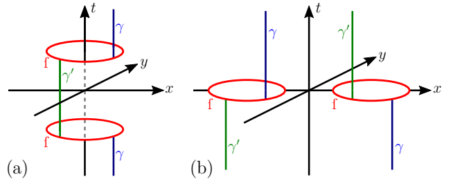
FIG. 5. (a) is an illustration of a 2+1 Deutsch-Politzer spacetime, and (b) is an illustration of a 2+1 teleporter spacetime. In each case, the spacetimes are assumed to be flat everywhere except the surface \mathbb{f} , which contain a SCDS. Both \gamma and \gamma' are timelike curves [note that \gamma' in (a) is a closed timelike curve].
