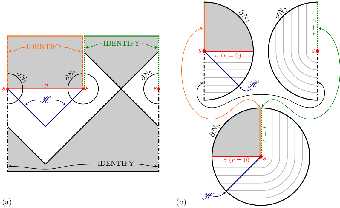
FIG. 4. Neighborhood of a d + 1 dimensional black hole end point s on a surface \Sigma_\Omega . In (a), the neighborhood of s in the conformal diagram [cf. Fig. 3 (b)], is the region enclosed by the boundaries \partial N_i , i \in \{1, 2, 3\} . (b) is a detailed diagram of the neighborhood (identifications indicated by arrows) with the gray contours describing surfaces of constant areal radius r > 0 .
