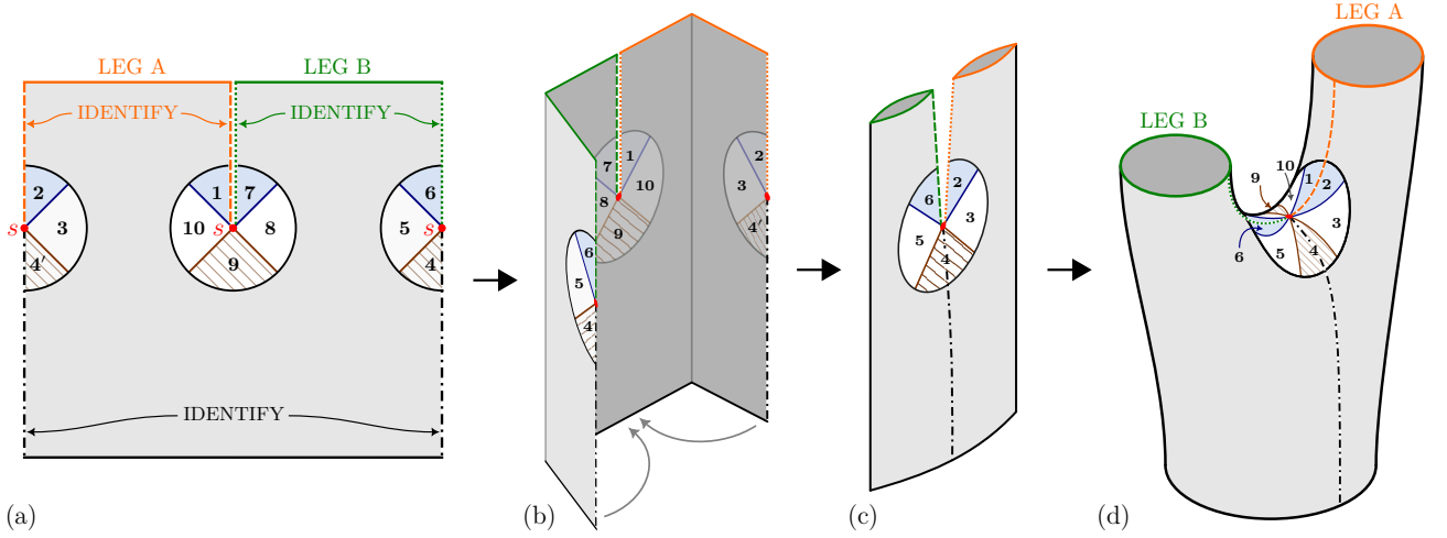
FIG. 2. (a) depicts a flat 1+1 trousers spacetime and the neighborhood N_s of the crotch singularity s , with the time direction oriented vertically. (b) and (c), respectively, illustrate a folding and gluing procedure to construct a paper model of a 1+1 trousers spacetime [observe that regions 4' and 4 of (a) and (b) have been combined into a single region 4 here to facilitate comparison with Fig. 1]. (d) illustrates a homeomorphic deformation of the 1+1 trousers spacetime to illustrate the neighborhood N_s more clearly. In all diagrams, the solid shaded regions of N_s indicate the future light cones of s , and the crosshatched regions indicate the past light cones of s .
