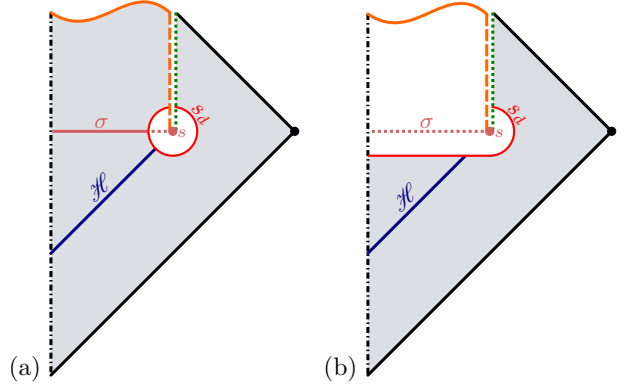
FIG. 7. Possible regularization scenarios for an evaporating black hole in an ELST. As in Figs. 3 and 4, \mathcal{H} is the horizon, and \sigma and s indicate where the respective Schwarzschild and end point singularities would otherwise be. The effective metric \mathbf{g}_{ab} is Lorentzian in the shaded regions, and the red contour s_d is the surface where \mathbf{g}_{ab} becomes degenerate.
