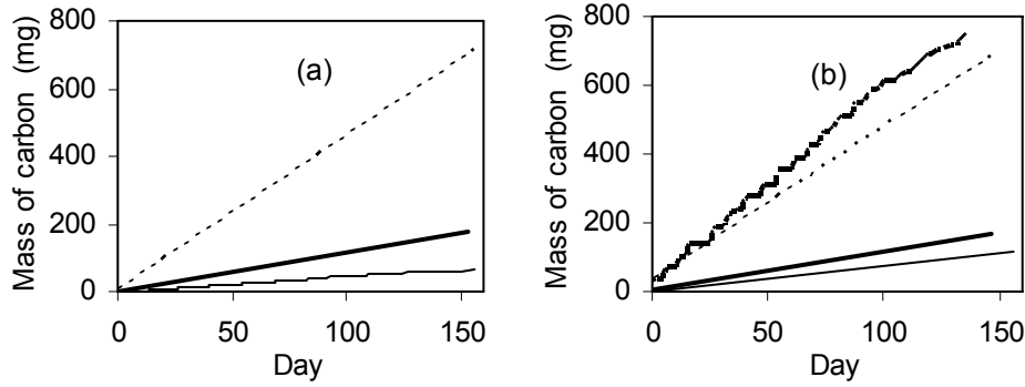
Fig. 4.15 Variation of the cumulative mass of T-C (thin dashed line) & TOC (thick solid line) applied on the column via influent, and the cumulative mass of T-C (thick dashed line) and TOC (thin solid line) discharged as E in (a) CA and (b) IA (high porous soil).
