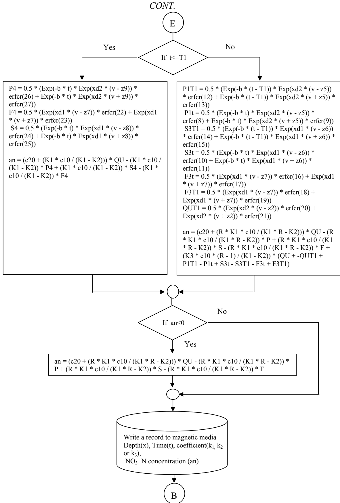
Fig. C-2 Flow chart of the computer program developed to compute NO 3 - -N for a given data set of t and x , using a given range of k_1 or k_2 for CA of low porous soil.
