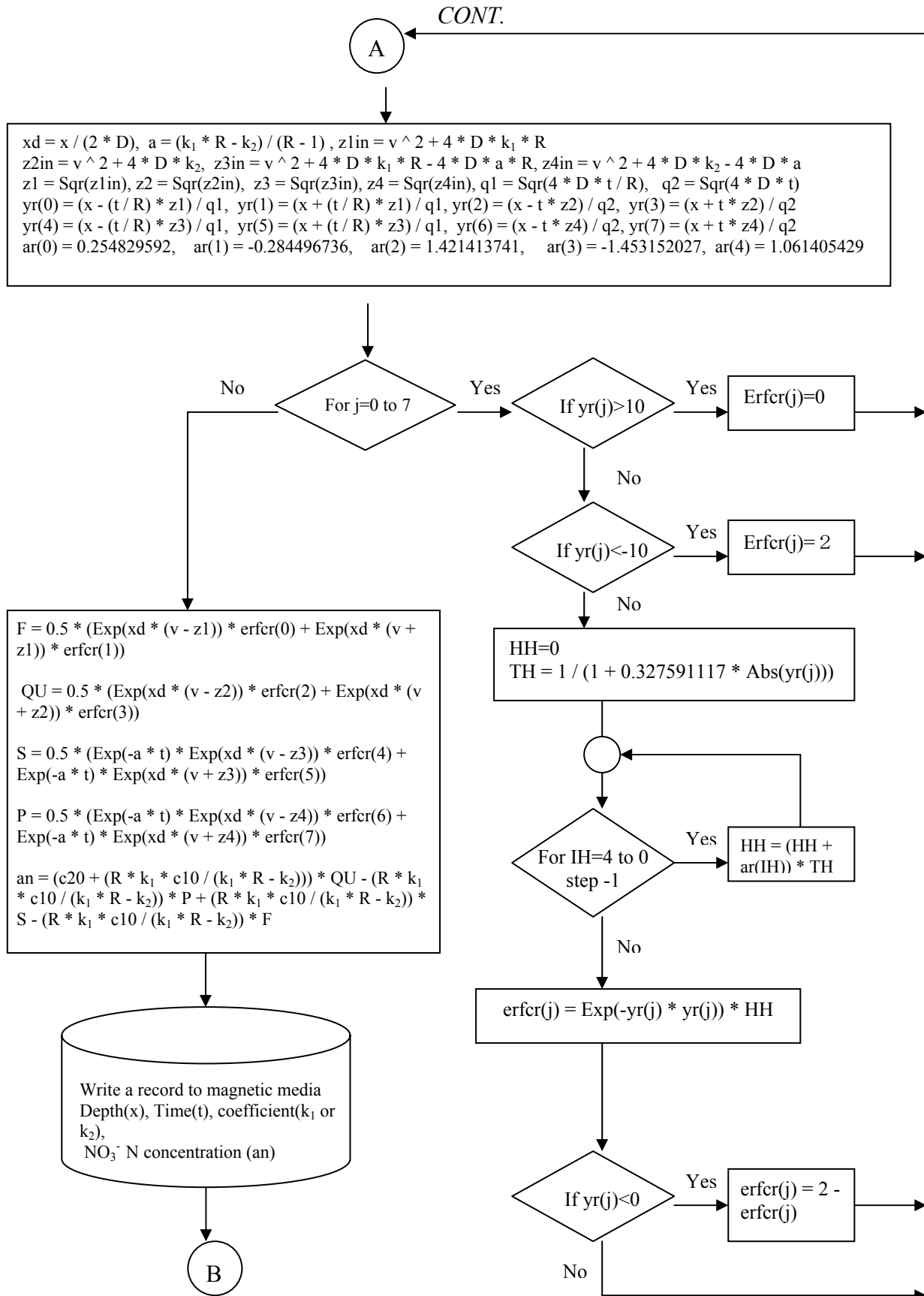
Fig. C-1 Flow chart of the computer program developed to compute \text{NO}_3^- -N for a given data set of t and x , using a given range of k_1 or k_2 for CA of high porous soil.
