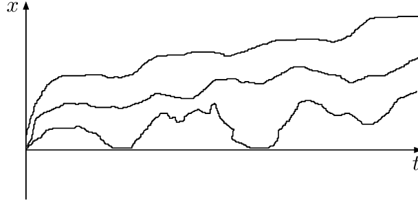
Figure 6. Dyson's BM with a reflective boundary
