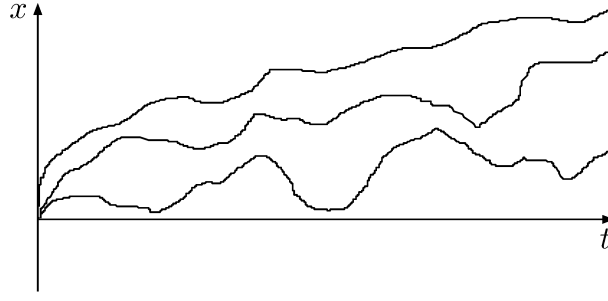
Figure 5. Dyson's BM with an absorbing boundary
