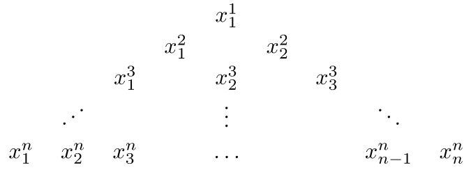
Figure 3. Gelfand-Tsetlin cone
