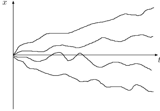
Figure 1. Dyson's BM
