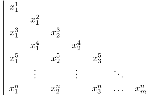
Figure 7. Symplectic Gelfand-Tsetlin cone.
