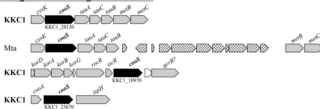
Fig. 2-4. Schematic representation of CooS gene clusters from C. maritimus KKC1, M. thermoacetica , M. perchloratireducens , C. subterraneus subsp. pacificus , and C. hydrogenoformans . KKC1, C. maritimus ; Mta, M. thermoacetica ; Mpe, M. perchloratireducens ; Csp, C. subterraneus subsp. pacificus ; Chy, C. hydrogenoformans ; Gsu, Geobacter sulfurreducens . Black, cooS ; dots, inserted genes; gray, other functional proteins.
