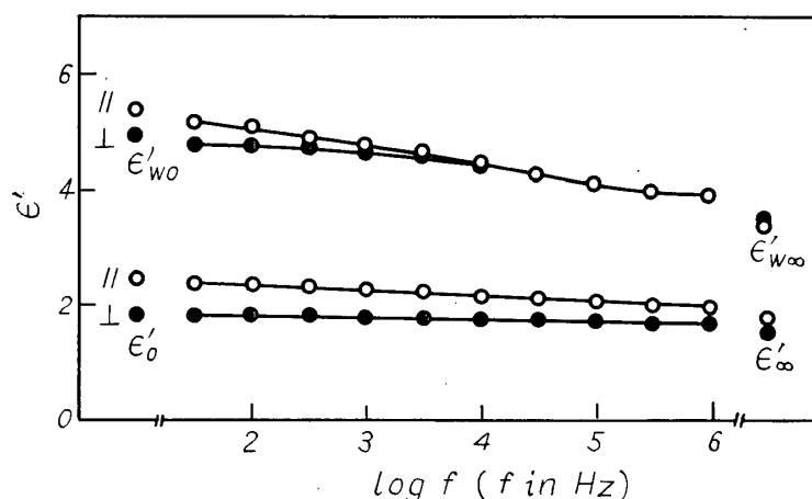
Fig. 10. The dielectric constants of western hemlock and wood substance in parallel and perpendicular to grain at -58^{\circ}\text{C} as a function of frequency.
