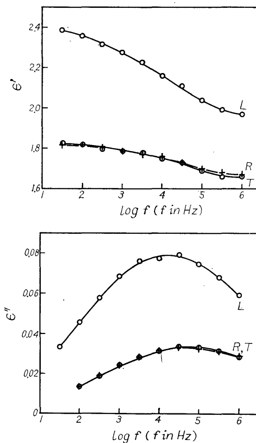
Fig. 8. The dielectric dispersion and absorption curves for western hemlock in L, R and T directions at -58^\circ\text{C} .
