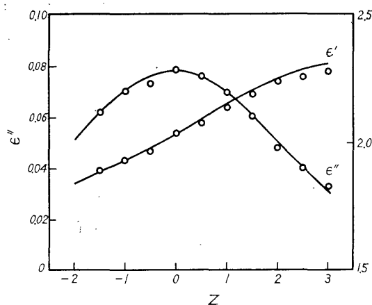
Fig. 23. The comparison of experimental values with calculated values (equations (30) and (31)) for dielectric constant and dielectric loss factor of Hoonoki in L direction at -58^{\circ}\text{C} . \circ : experimental, —: calculated
