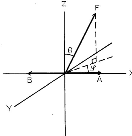
Fig. 16. The coordinate system used in the calculation of the complex dielectric constant of wood.
