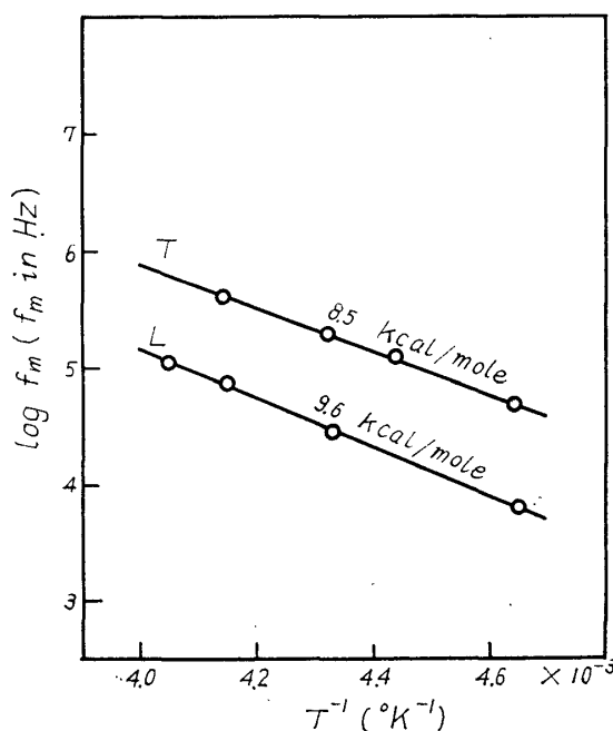
Fig. 25. \log f_m vs. T^{-1} curves for Keyaki in L and T directions.
