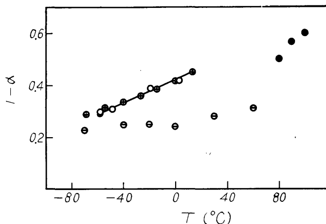
Fig. 14. The relationship between the parameter (1-\alpha) and temperature for wood and cellulose.
