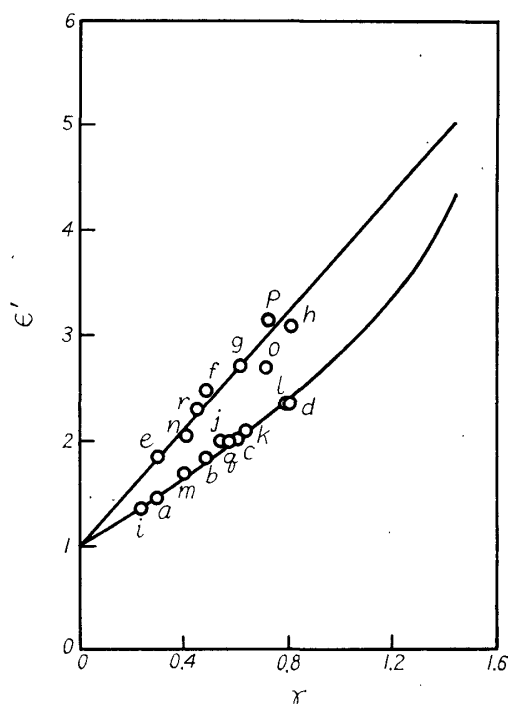
Fig. 9. The relationship between dielectric constant and specific gravity.
