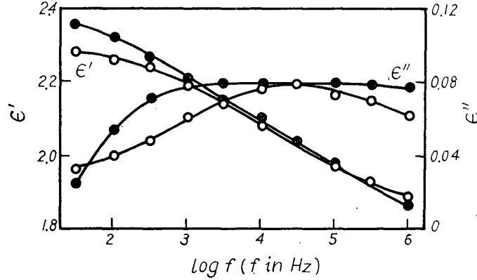
Fig. 17. The dielectric dispersion and absorption curves for Hoonoki.
