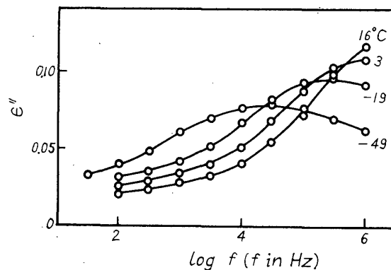
Fig. 2. The dielectric absorption curves for Hoonoki in L direction at respective temperatures.
